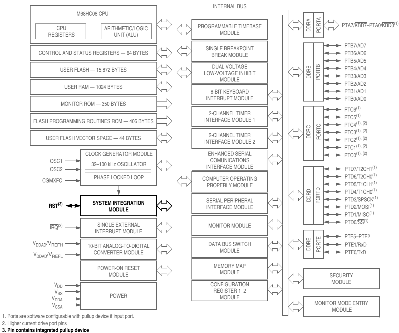
Figure 15-1. Block Diagram Highlight SIM Block and Pins
