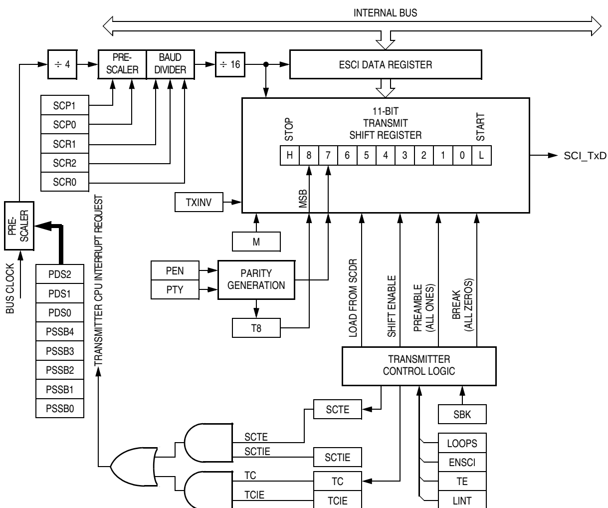
Figure 14-5. ESCI Transmitter
