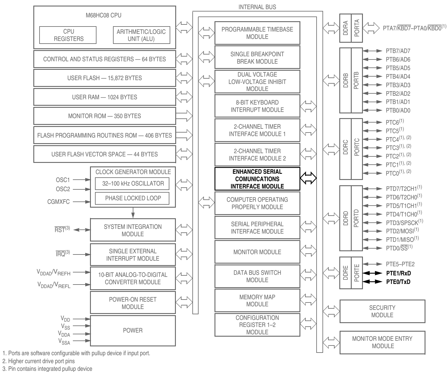
Figure 14-1. Block Diagram Highlighting ESCI Block and Pins
