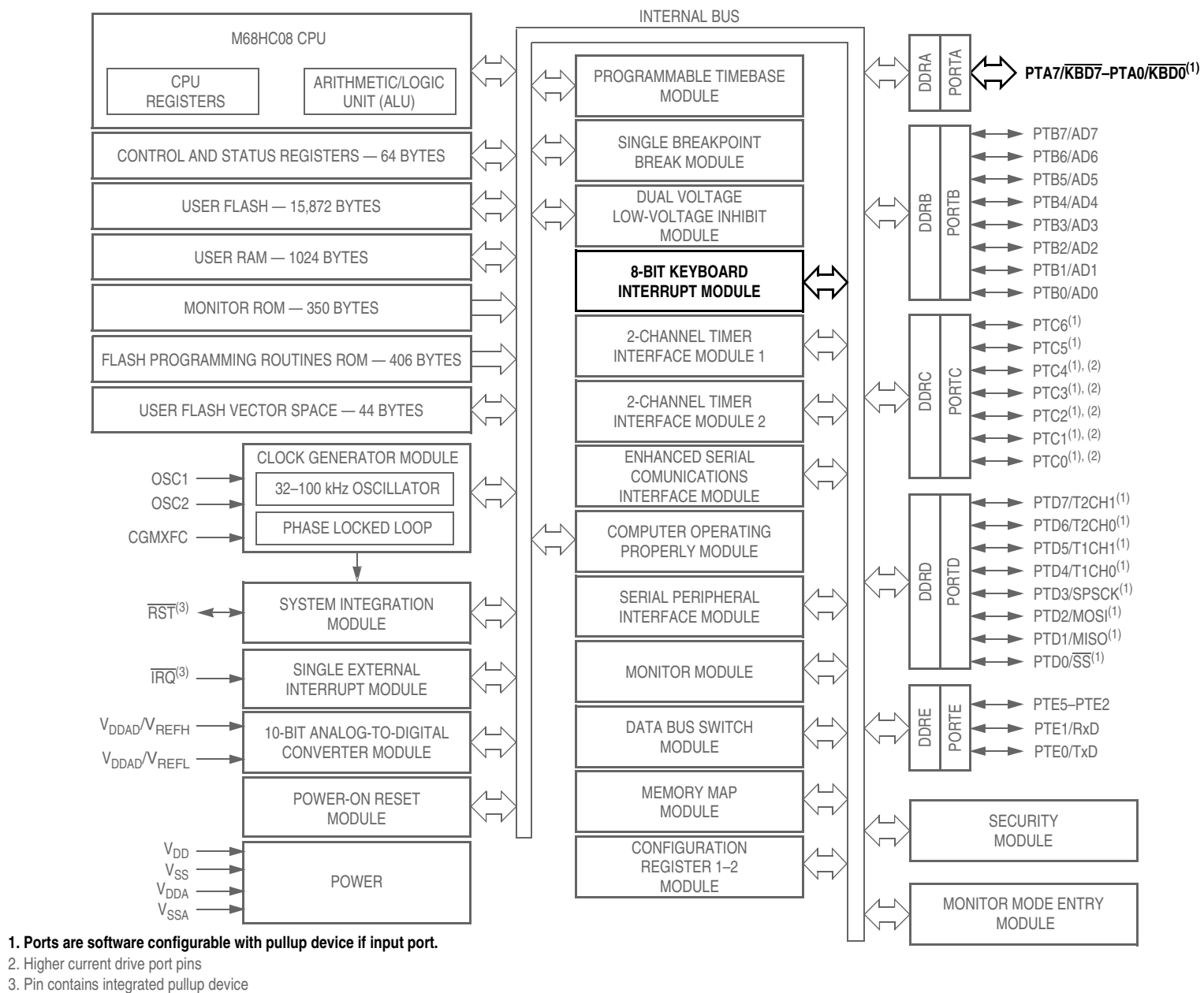
Figure 9-1. Block Diagram Highlighting KBI Block and Pins
