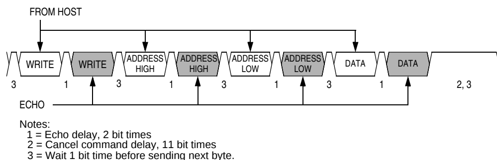
Figure 19-16. Write Transaction
