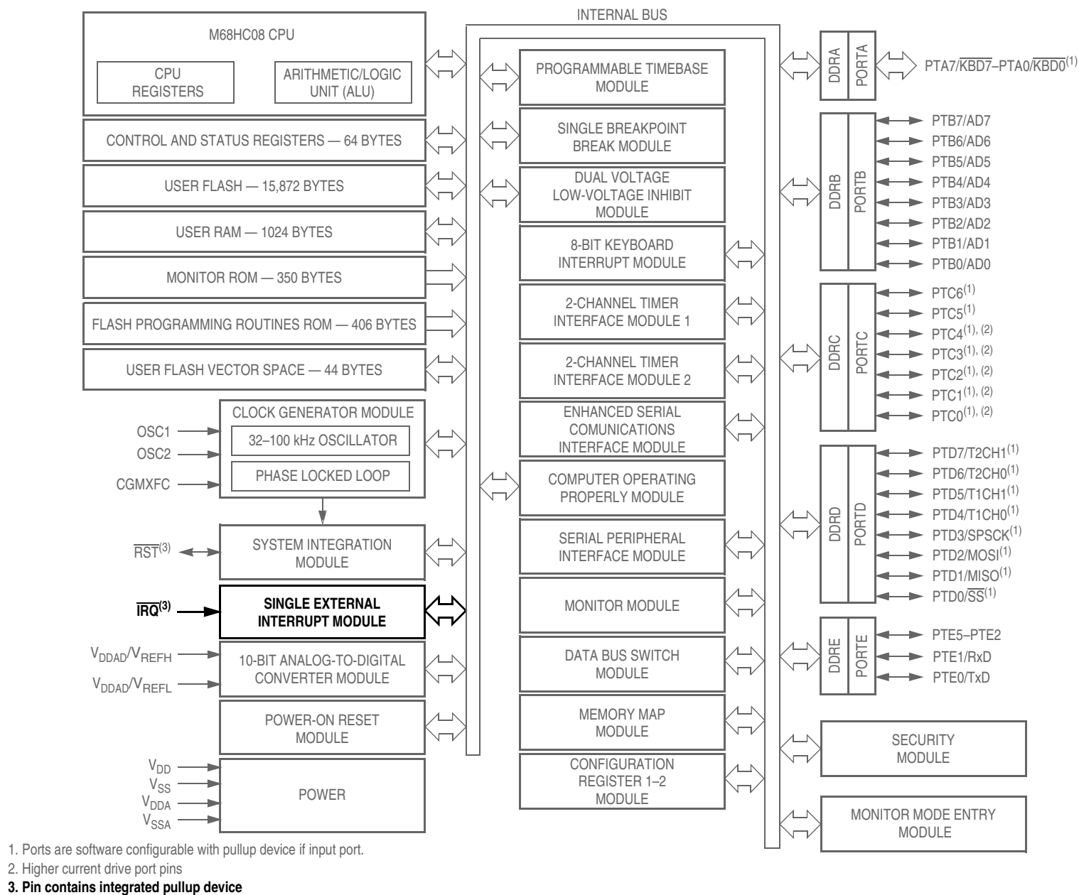
Figure 8-1. Block Diagram Highlighting IRQ Block and Pins
