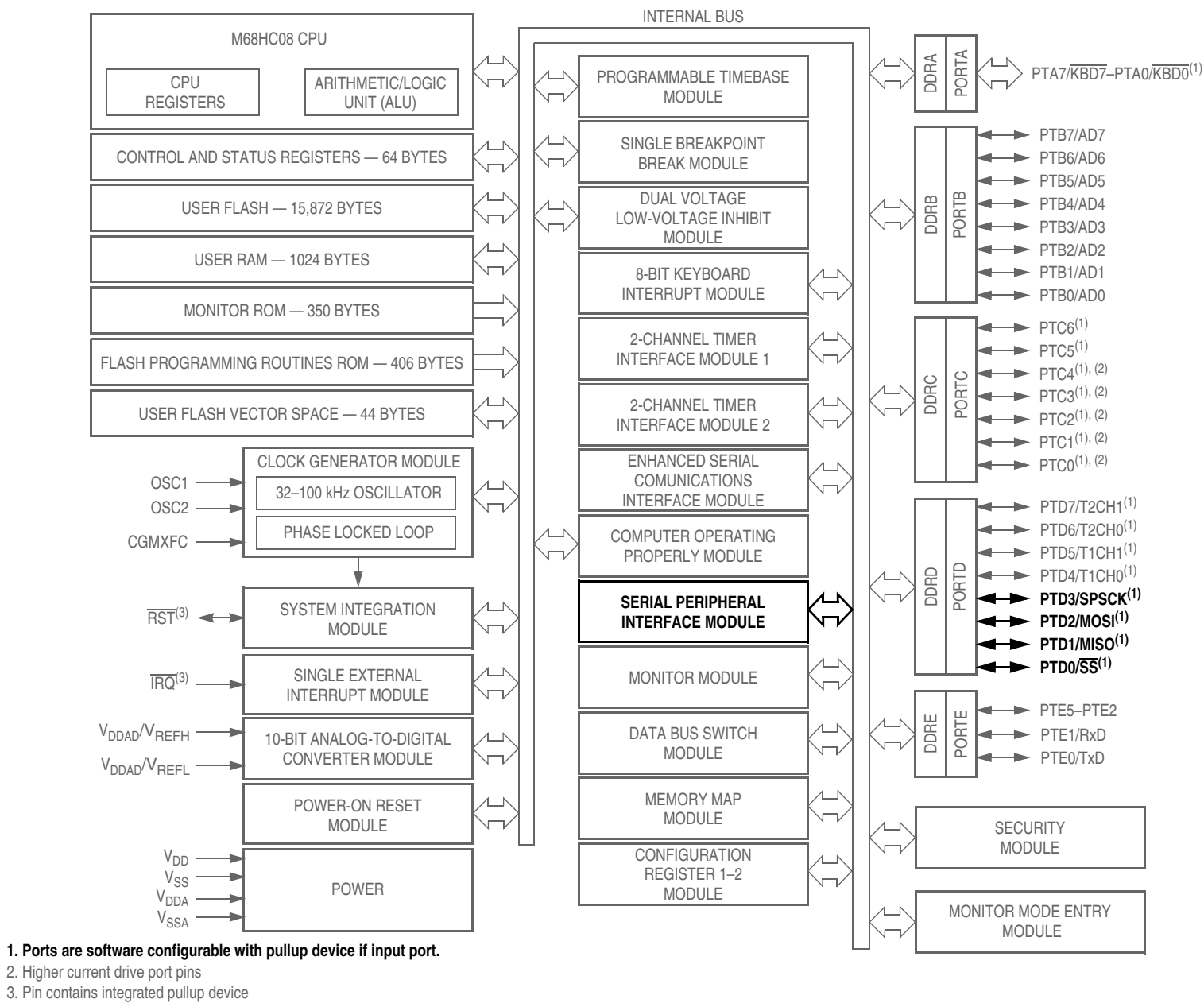
Figure 16-1. Block Diagram Highlighting SPI Block and Pins
