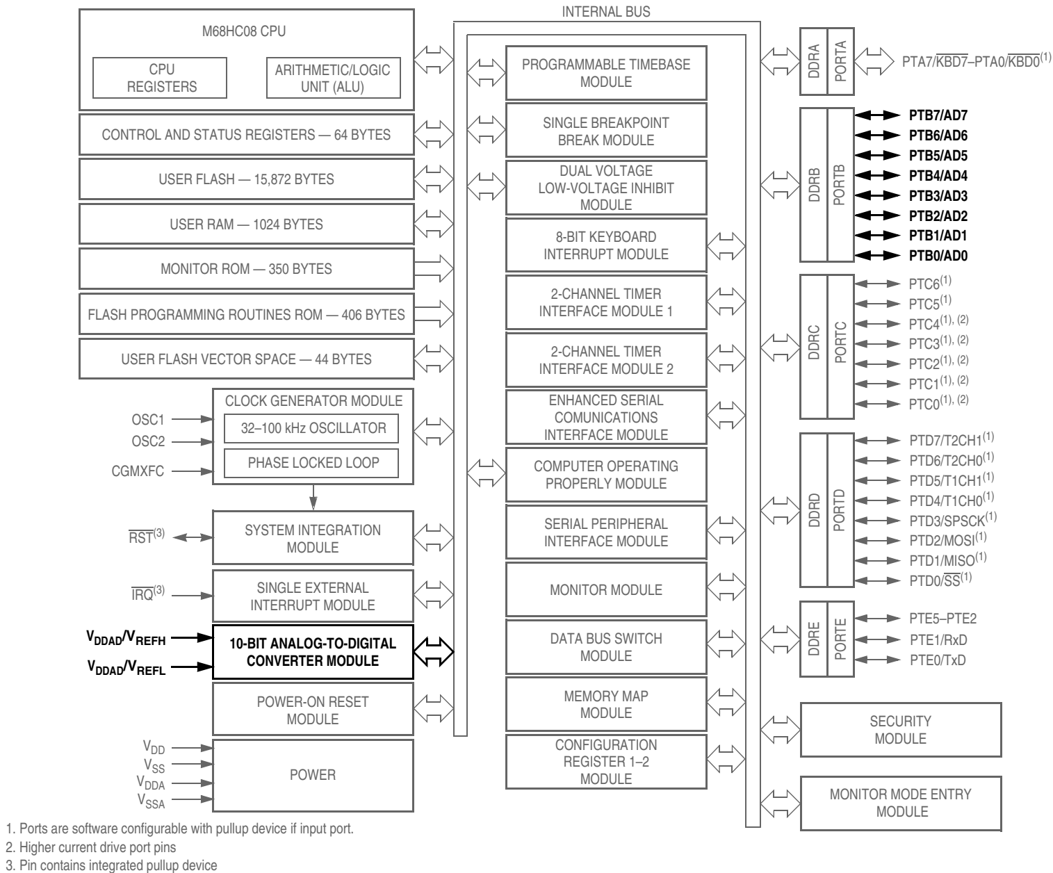
Figure 3-1. Block Diagram Highlighting ADC Block and Pins
