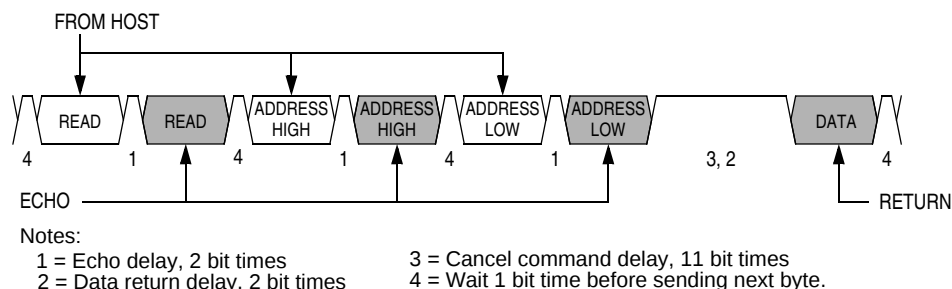
Figure 19-15. Read Transaction
