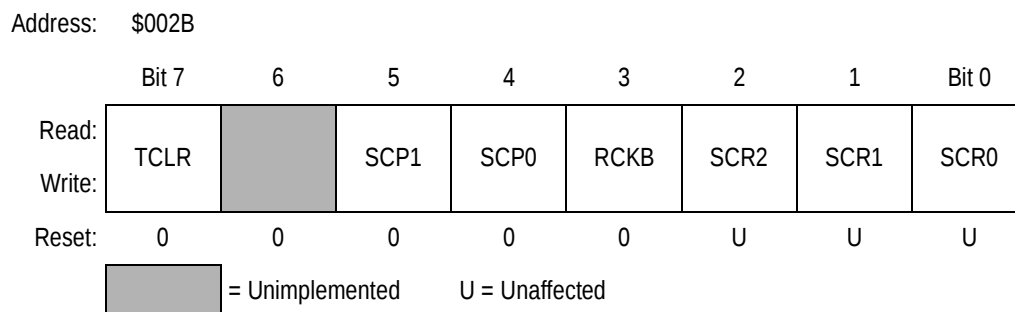
Figure 7-3. Baud Rate Register (BAUD)
