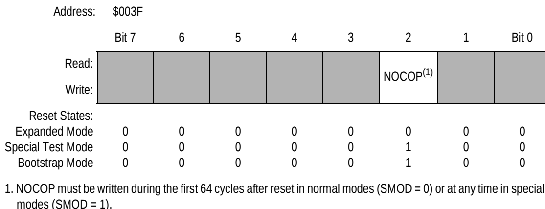
Figure 5-3. System Configuration Register (CONFIG)
