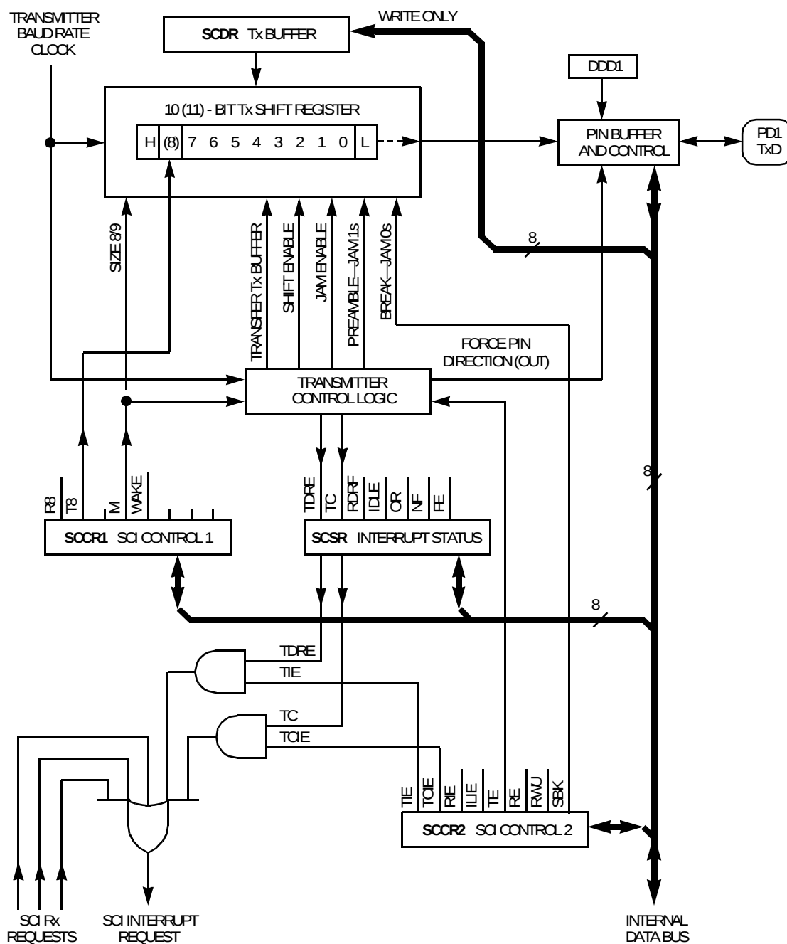
Figure 7-1. SCI Transmitter Block Diagram
