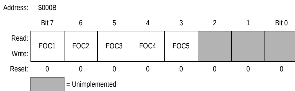
Figure 9-2. Timer Compare Force Register (CFORC)
