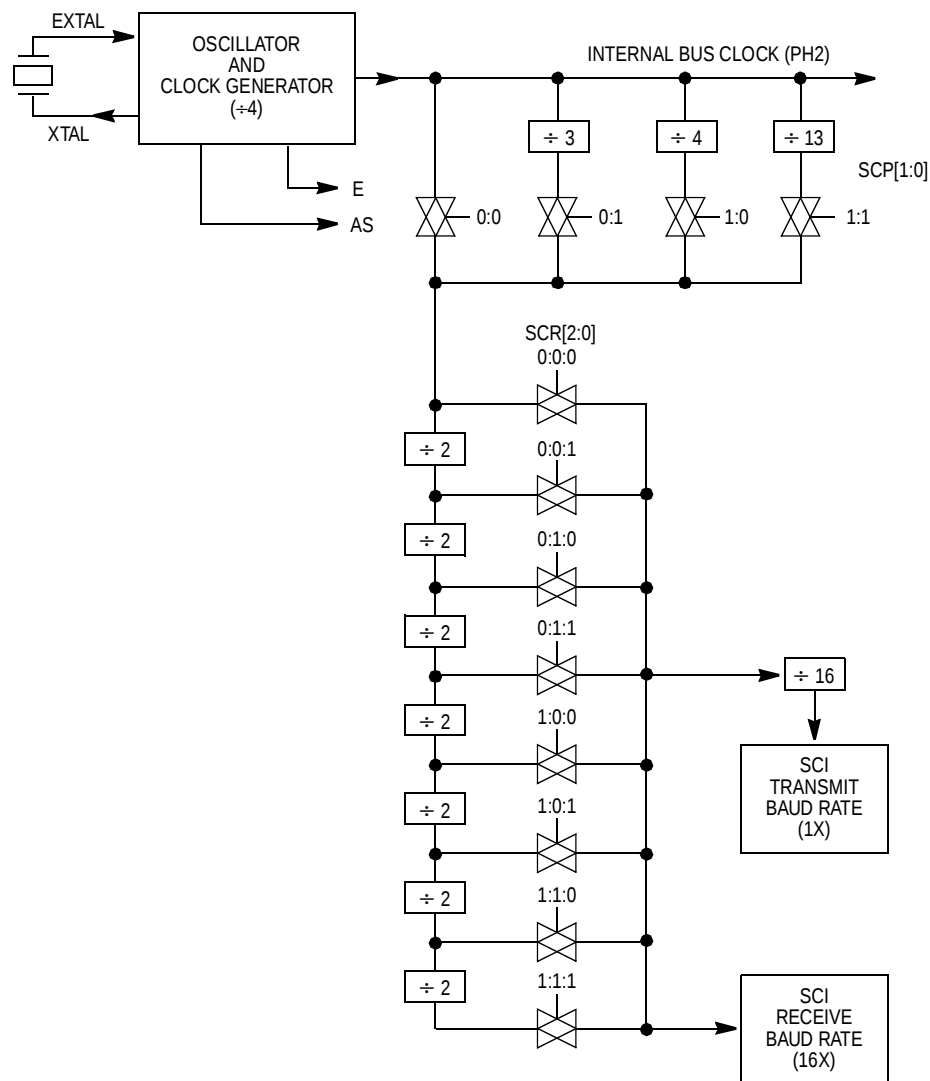
Figure 7-4. SCI Baud Rate Generator Clock Diagram
