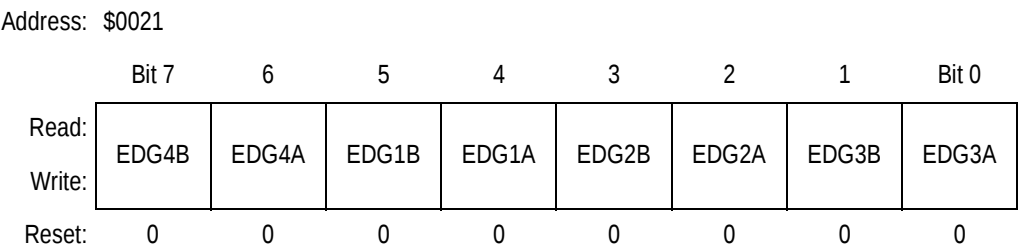
Figure 9-15. Timer Control Register 2 (TCTL2)
