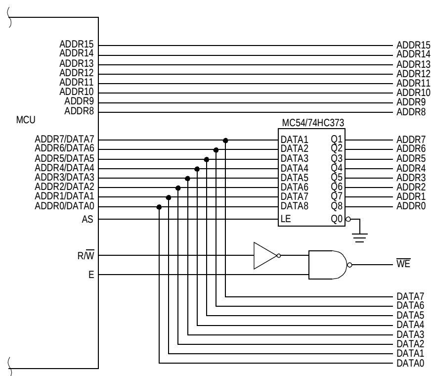
Figure 4-1. Address and Data Demultiplexing
