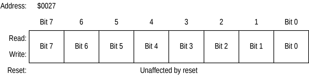
Figure 9-22. Pulse Accumulator Counter Register (PACNT)
