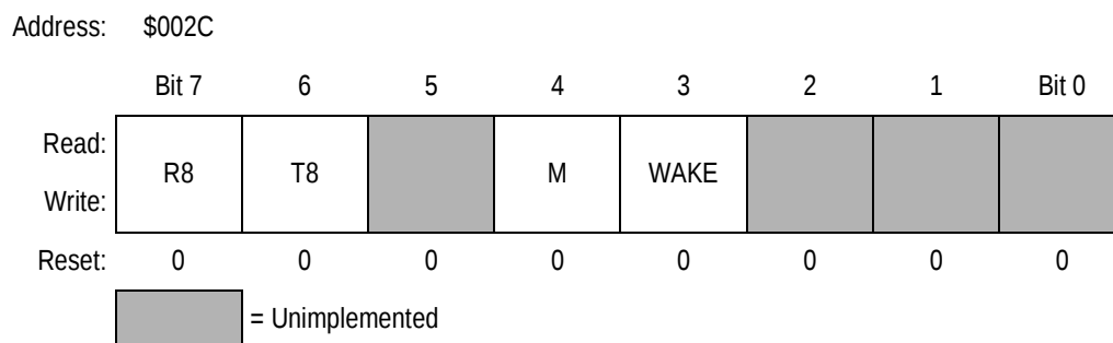
Figure 7-5. Serial Communications Control Register 1 (SCCR1)
