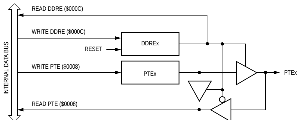
Figure 11-13. Port E I/O Circuit
