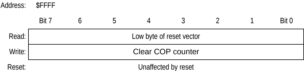
Figure 14-3. COP Control Register (COPCTL)
