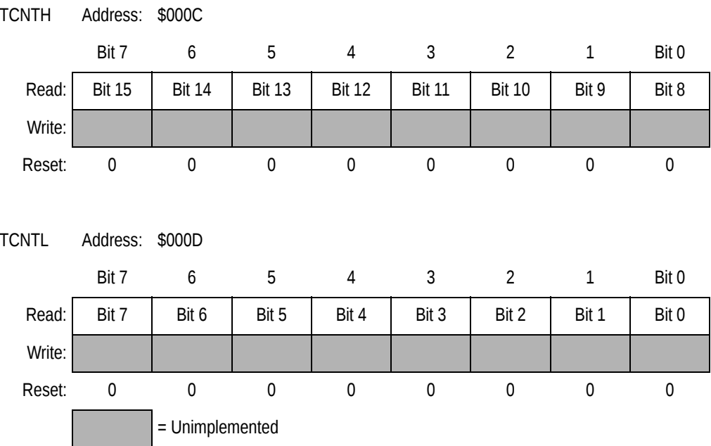
Figure 10-5. TIM Counter Registers (TCNTH:TCNTL)
