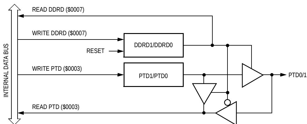
Figure 11-10. Port D I/O Circuit
