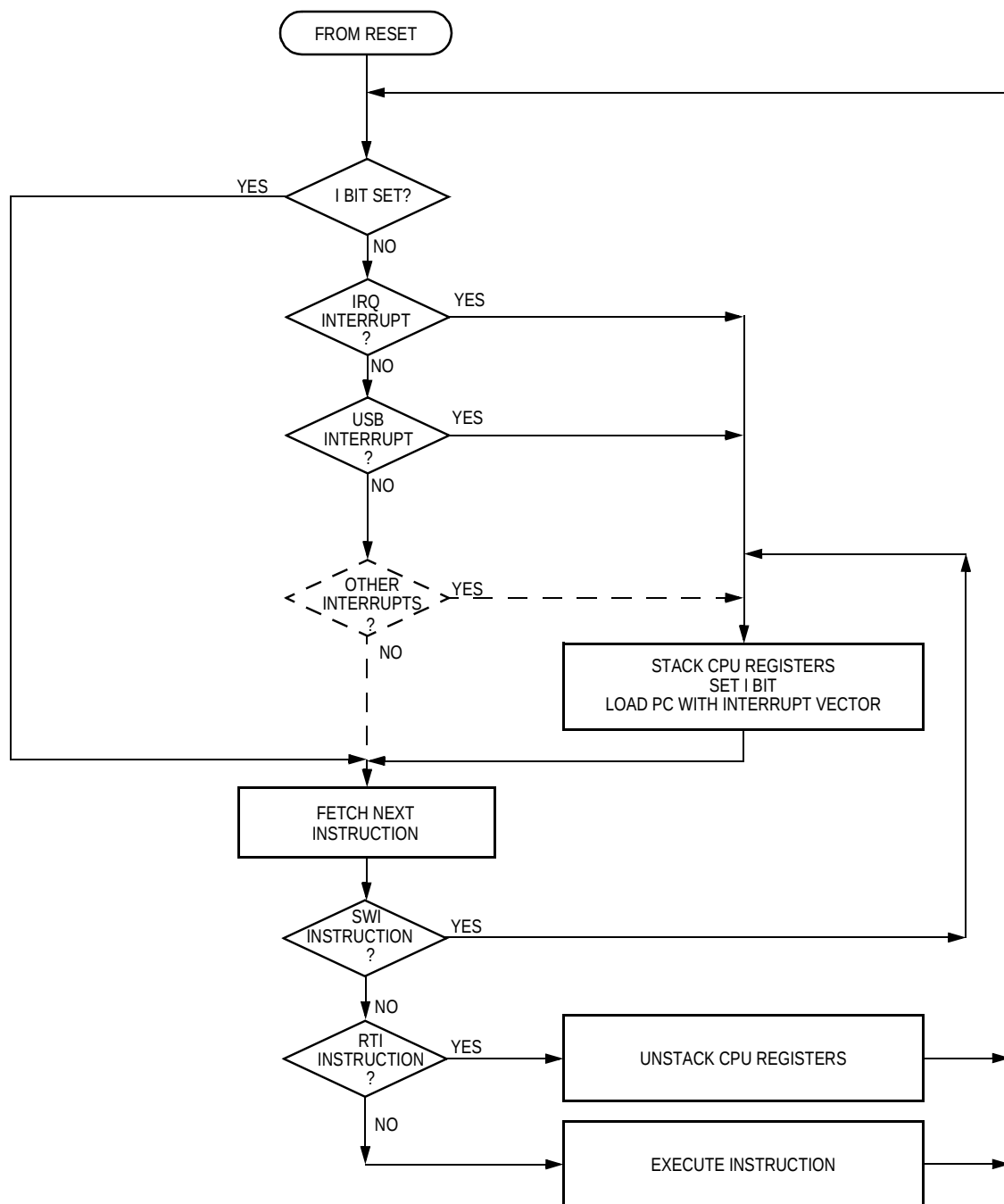
Figure 8-8. Interrupt Processing
