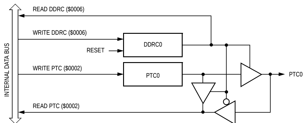
Figure 11-7. Port C I/O Circuit
