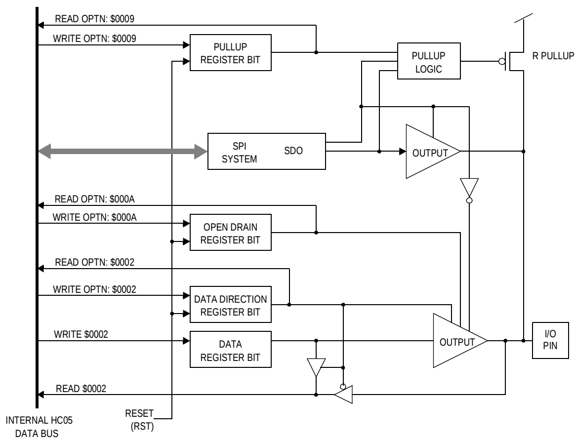
Figure 7-14. PC1/SDO Circuitry
