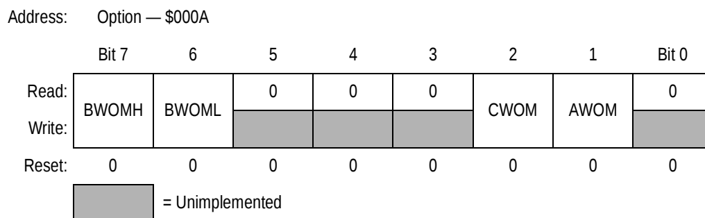
Figure 7-21. Wired-OR Mode Register (WOM)
