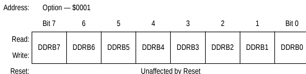
Figure 7-12. Port B Data Direction Register (DDRB)
