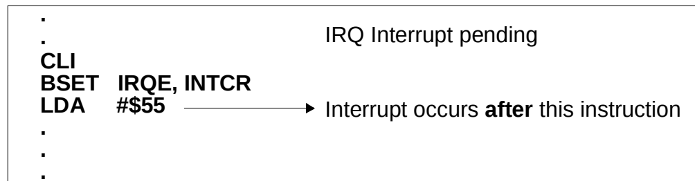
Figure 6-5. IRQ Timing Delay
