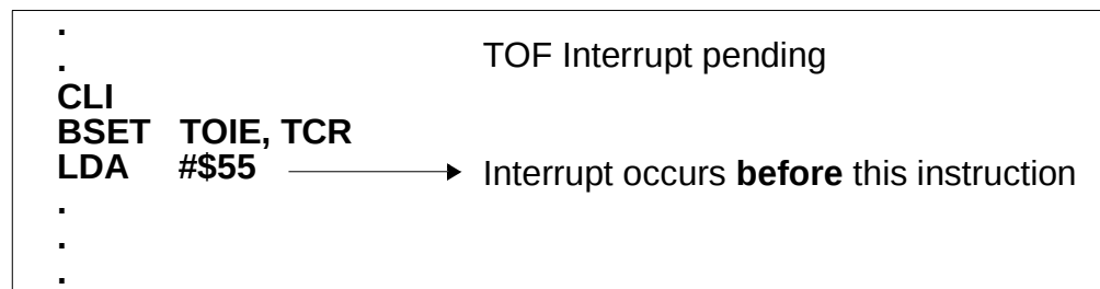
Figure 6-4. Timer Interrupt
