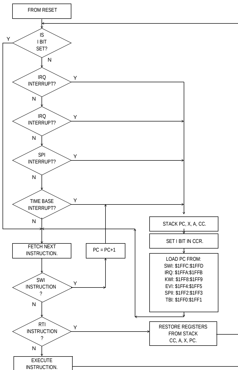
Figure 6-1. Interrupt Processing Flowchart
