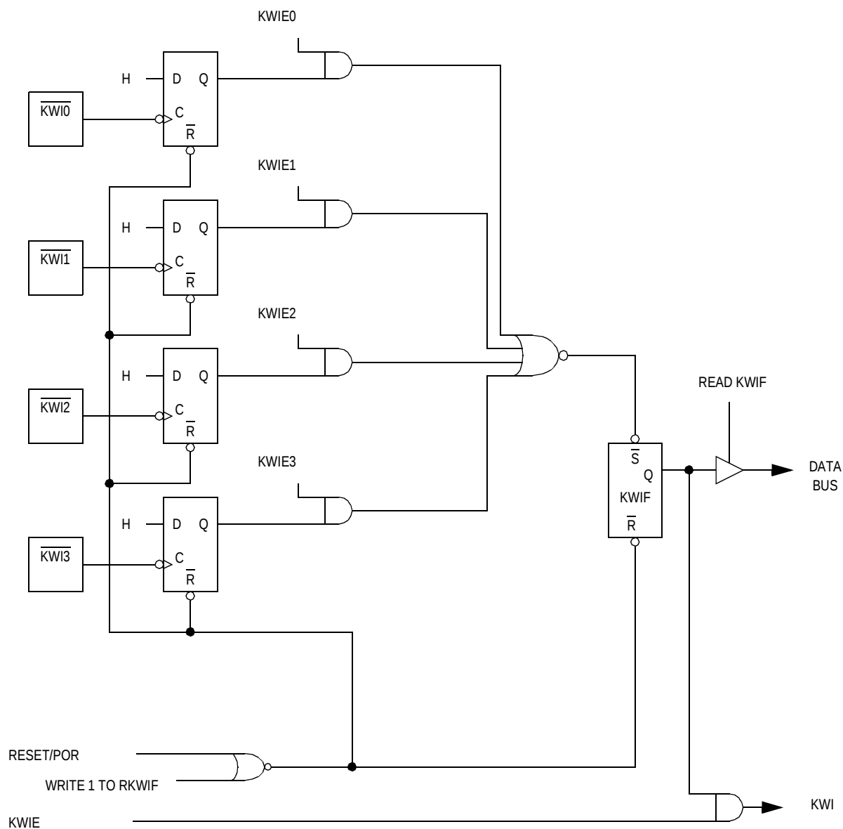
Figure 7-9. Key Wakeup Interrupt (KWI)
