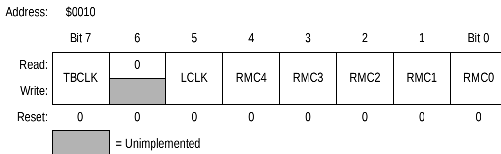
Figure 9-5. Time Base Control Register 1 (TBCR1)
