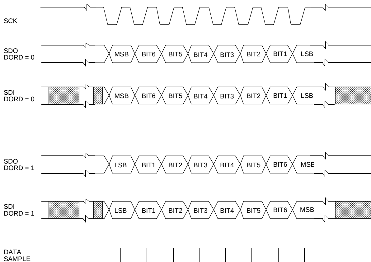
Figure 10-5. Clock/Data Timing
