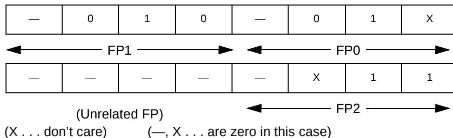
Figure 11-9. 1/3 Duty Example
