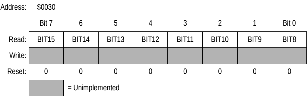
Figure 13-6. Event Counter Data High Register (EVDH)
