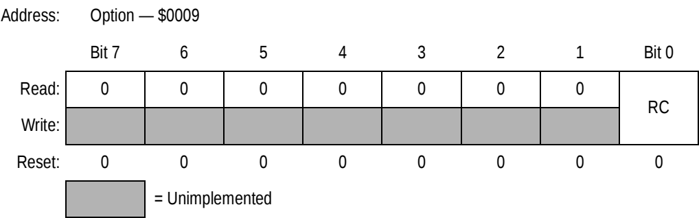
Figure 7-20. Resistor Control Register 2 (RCR2)
