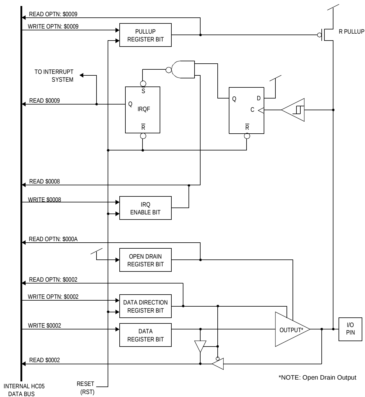
Figure 7-16. PC3/ \overline{\text{IRQ}} Circuitry
