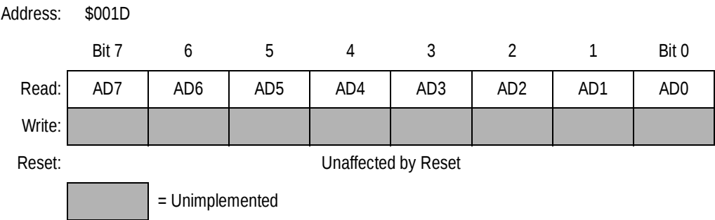
Figure 12-2. A/D Conversion Value Data Register (ADDR)
