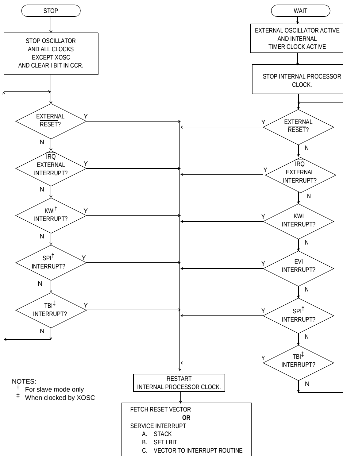
Figure 3-1. Stop/Wait Flowcharts
