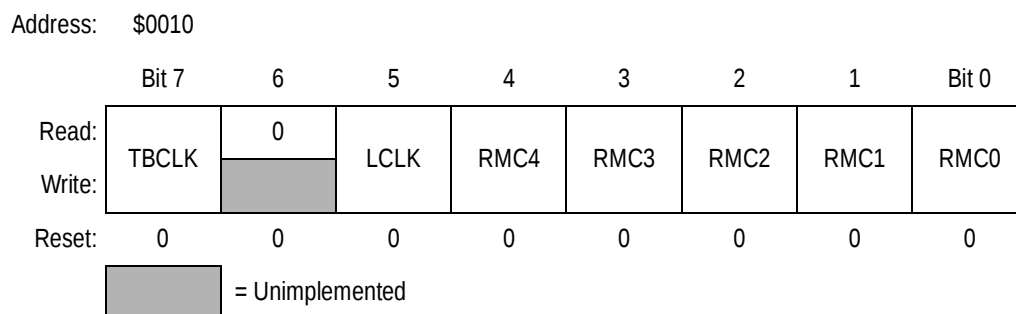
Figure 11-14. Time Base Control Register 1 (TBCR1)
