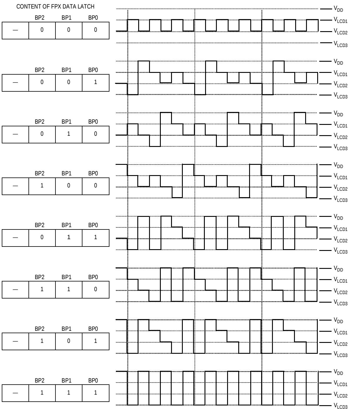
Figure 11-7. 1/3 Duty LCD Frontplane Driver Waveforms
