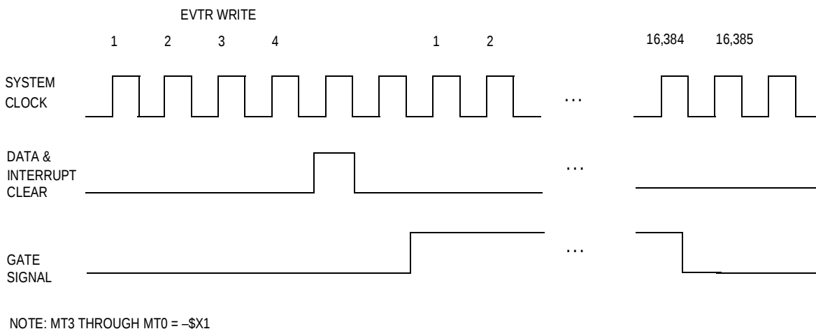
Figure 13-5. Event Counter Gate Signal Timing Example
