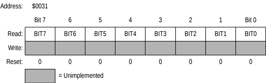
Figure 13-7. Event Counter Data Low Register (EVDL)
