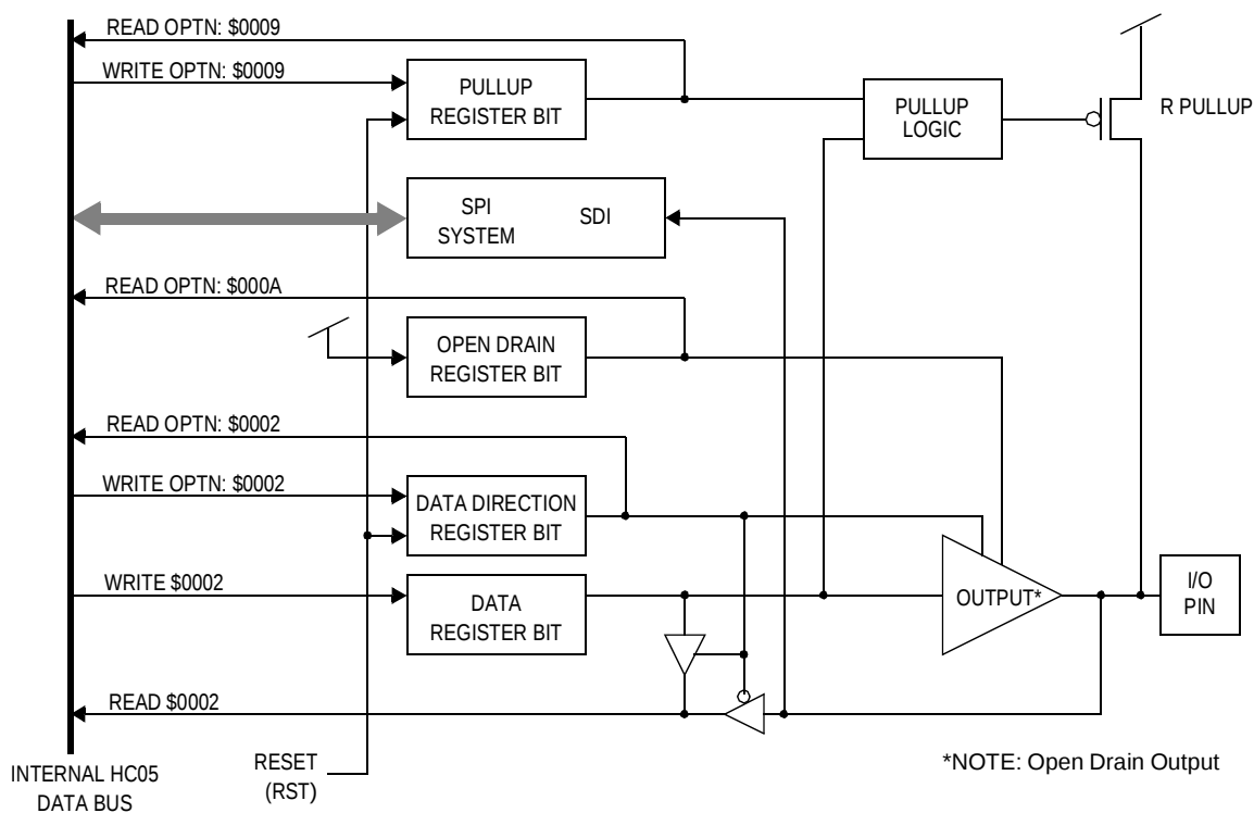
Figure 7-15. PC2/SDI Circuitry
