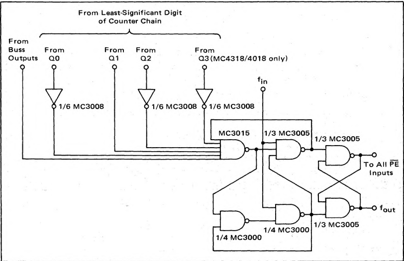
FIGURE 2 – FREQUENCY EXTENDER
