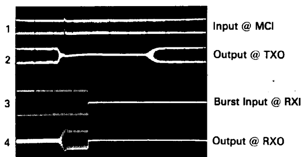
FIGURE 17 — IDLE-RECEIVE SWITCHING
