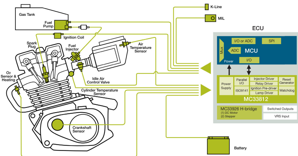
MC33812 Simplified Application Drawing
