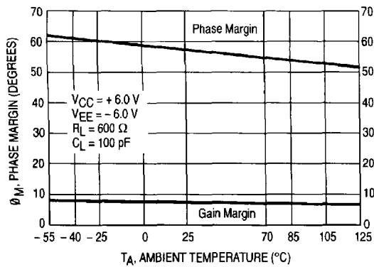
Figure 20. Gain and Phase Margin versus Temperature
