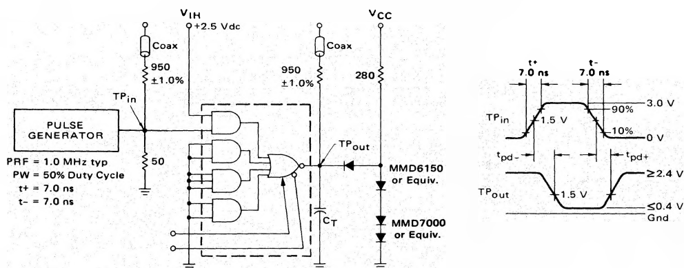
SWITCHING TIME TEST CIRCUIT AND WAVEFORMS
