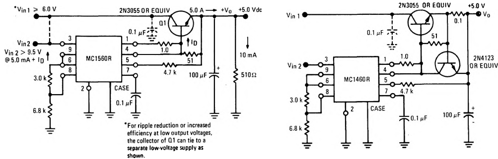
FIGURE 18 – NPN CURRENT BOOST CIRCUITS
