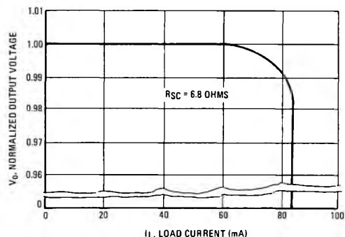
FIGURE 6 – CURRENT-LIMITING CHARACTERISTICS
