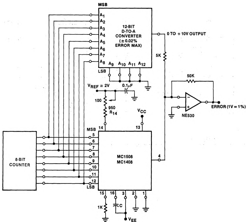
Figure 3. Relative Accuracy
