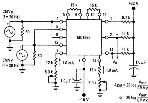
FIGURE 6 – COMMON MODE INPUT VOLTAGE AND GAIN MEASUREMENT
