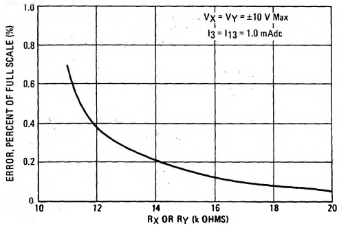
FIGURE 8A – ERROR CONTRIBUTED BY INPUT DIFFERENTIAL AMPLIFIER
