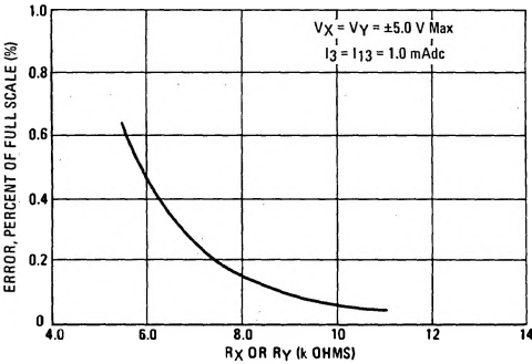
FIGURE 8B – ERROR CONTRIBUTED BY INPUT DIFFERENTIAL AMPLIFIER
