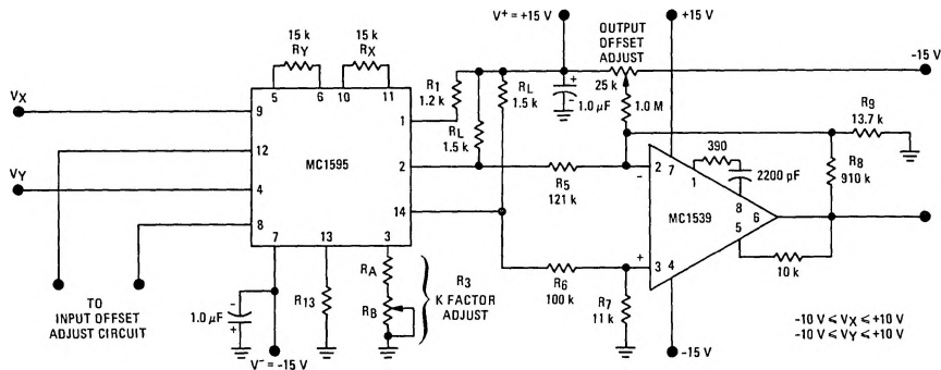
FIGURE 12 – MULTIPLY WITH DISCRETE LEVEL SHIFT
