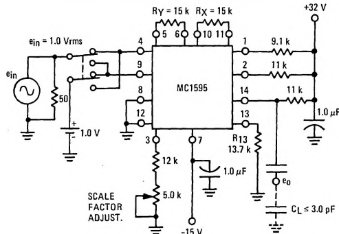
FIGURE 5 – BANDWIDTH MEASUREMENT
