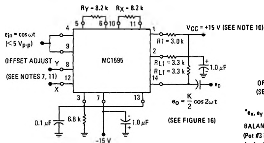
FIGURE 14 – FREQUENCY DOUBLER
