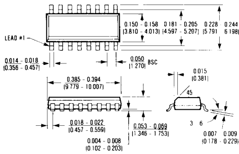
16 Lead Small Outline \theta_{JA} = 110^\circ\text{C/W} \theta_{JC} = 60^\circ\text{C/W}
