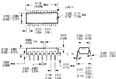
14 Lead Plastic DIP \theta_{JA} = 140^\circ\text{C/W} \theta_{JC} = 70^\circ\text{C/W}
