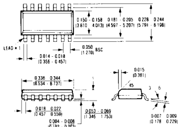
14 Lead Small Outline \theta_{JA} = 115^\circ\text{C/W} \theta_{JC} = 60^\circ\text{C/W}
