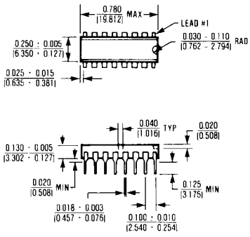
16 Lead Plastic DIP \theta_{JA} = 135^\circ\text{C/W} \theta_{JC} = 65^\circ\text{C/W}
