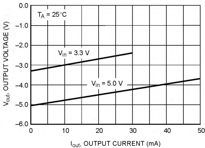
Figure 25. Voltage Inverter Load Regulation Output Voltage vs. Output Current MAX828
