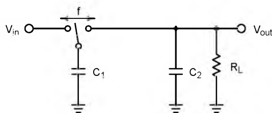
Figure 22. Ideal Switched Capacitor Model
