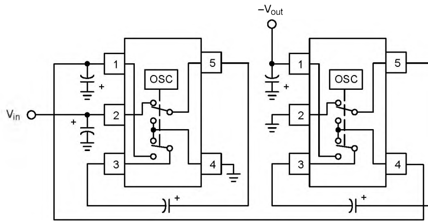
Figure 27. Cascade Devices for Increased Negative Output Voltage
