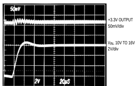
+3.3V LINE-TRANSIENT RESPONSE, RISING
