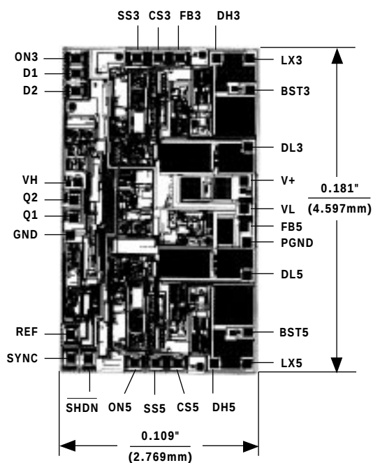
Chip Topography
