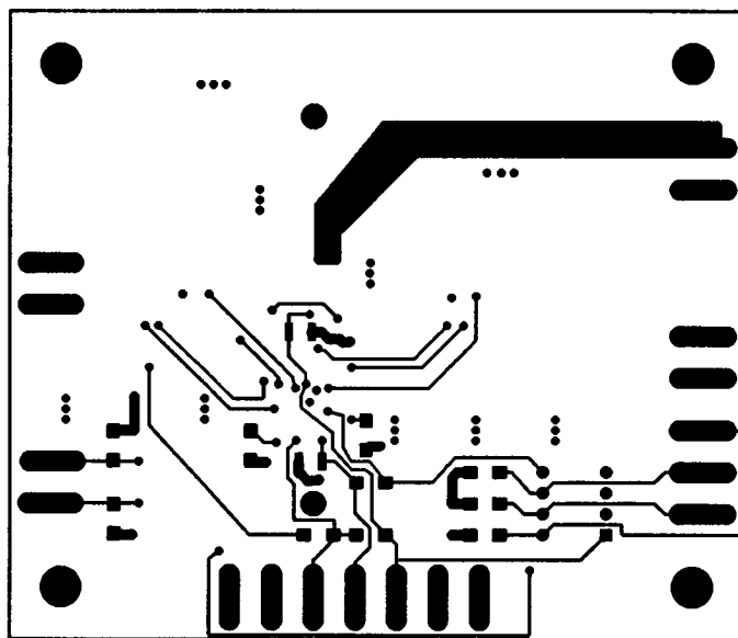
Figure 11. MAX786 EV Kit, Bottom Layer (Layer 4), Top View
