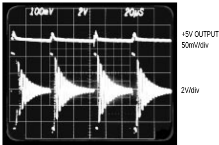
IDLE-MODE WAVEFORMS
