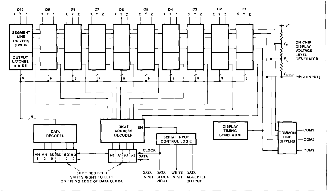
Figure 2. Block Diagram of MAX7232
