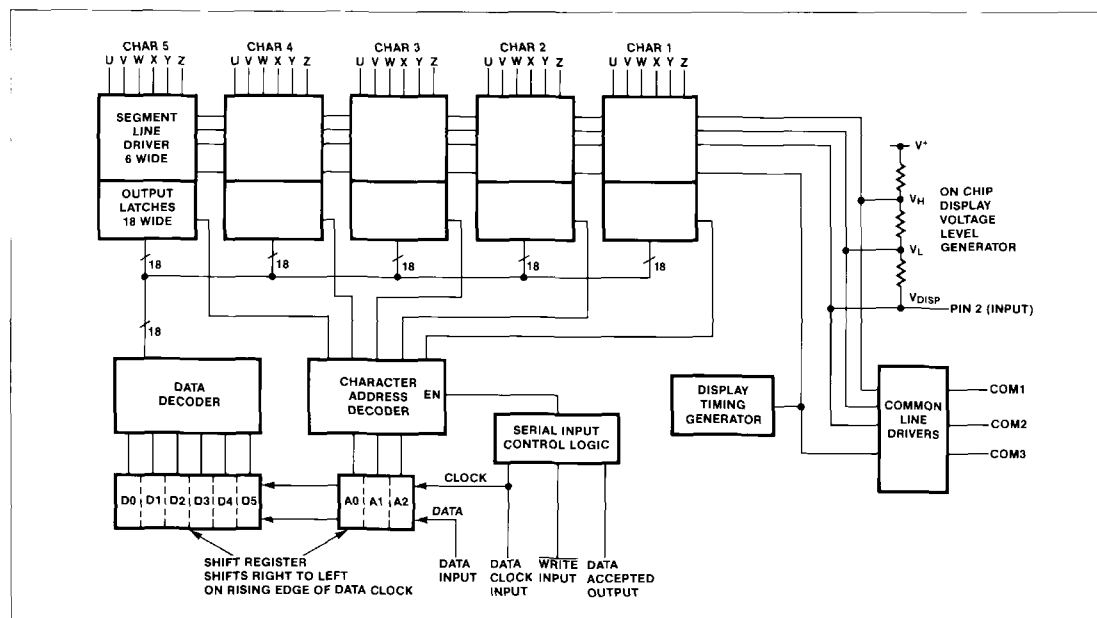
Figure 4. Block Diagram of MAX7234
