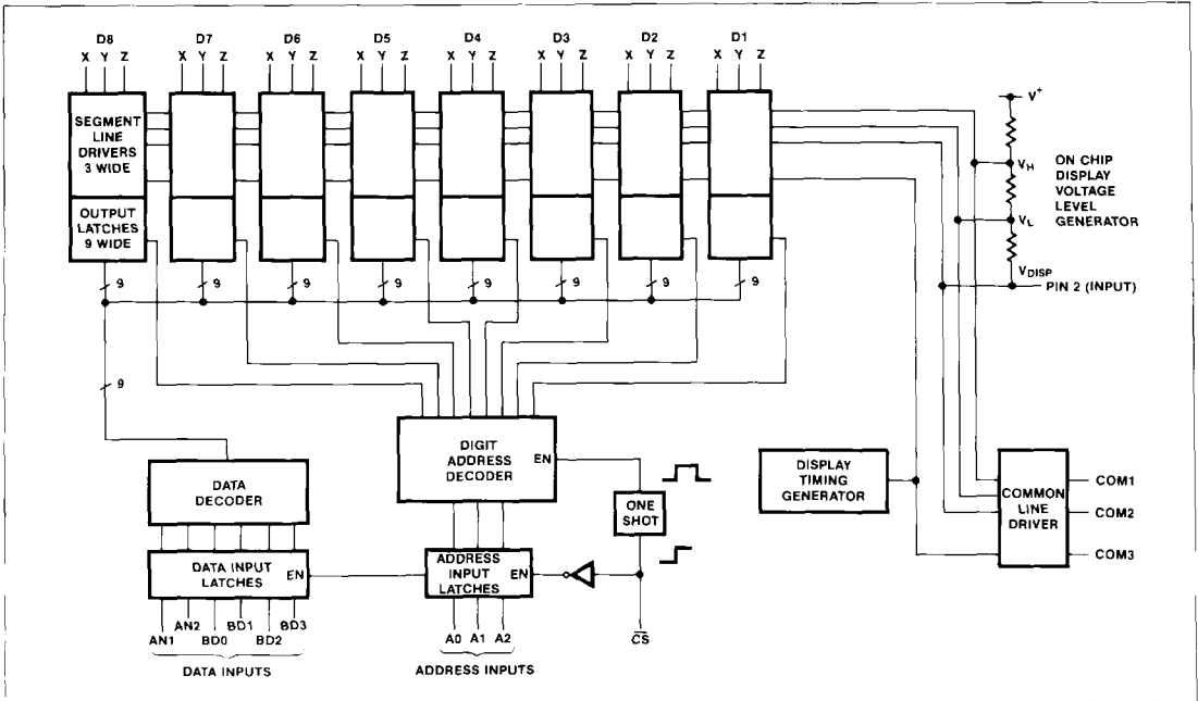
Figure 1. Block Diagram of MAX7231.
