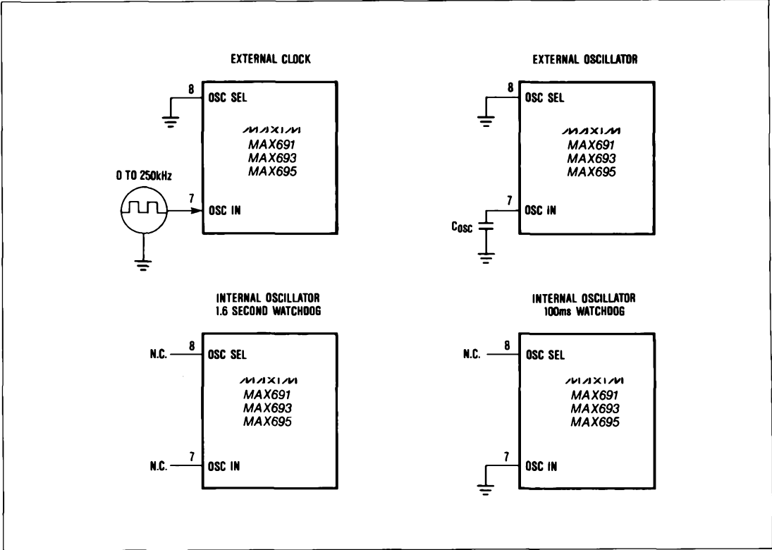
Figure 8. Oscillator Circuits
