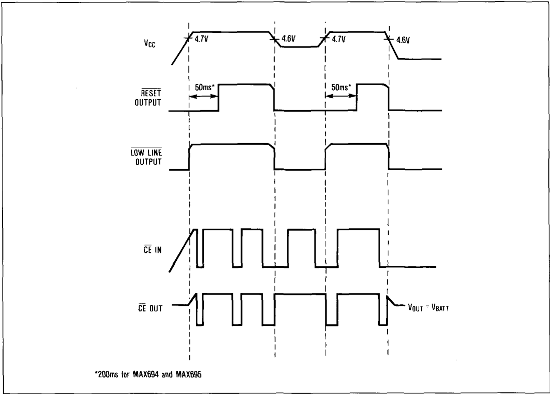
Figure 6. Reset Timing
