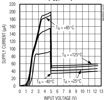
SUPPLY CURRENT vs. INPUT VOLTAGE ( V_{OUT} = 5V )
