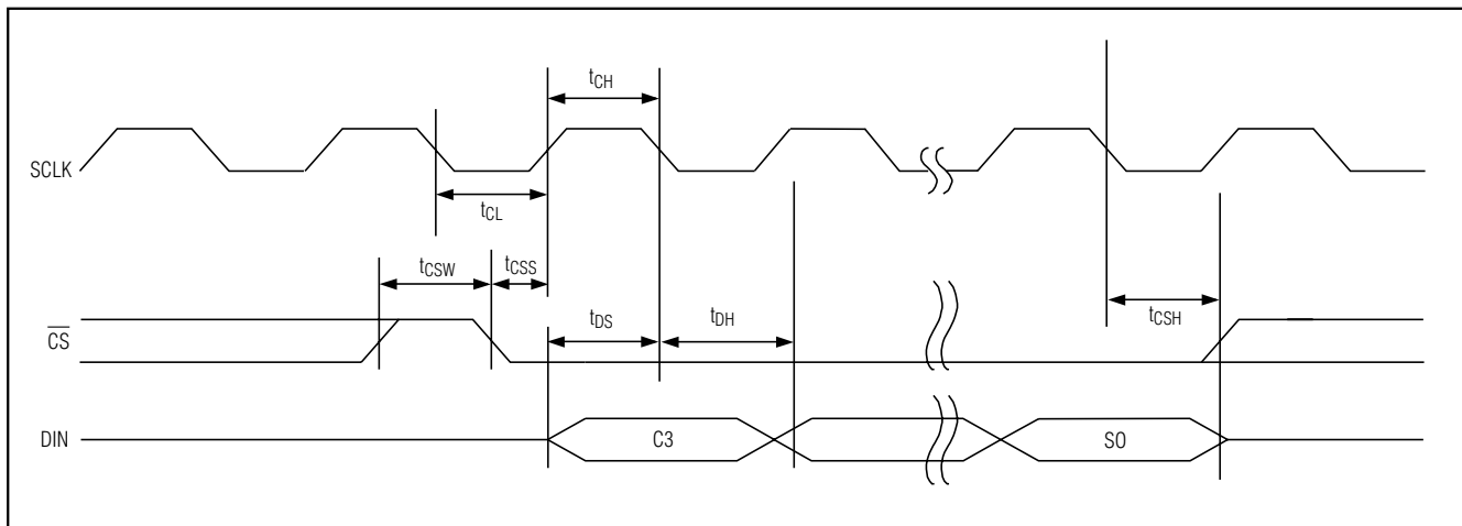
Figure 2. Timing Diagram
