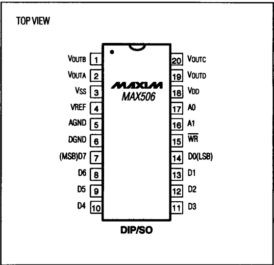
Pin Configurations (continued)
