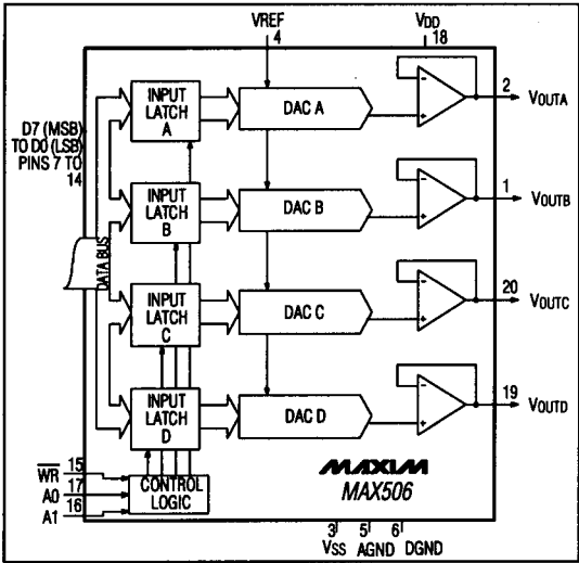
Functional Diagrams (continued)
