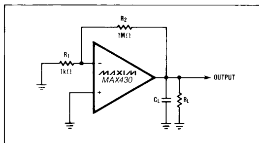
Figure 1. Test Circuit
