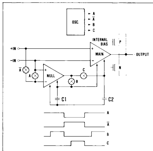
Figure 2. Maxim MAX430 Series Amplifier Block Diagram
