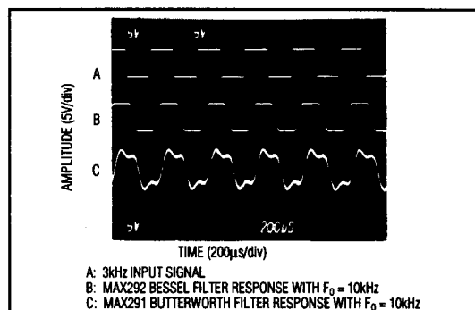
Figure 1. Bessel vs. Butterworth Filter Responses
