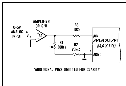
Figure 9. Full-Scale Adjustment
