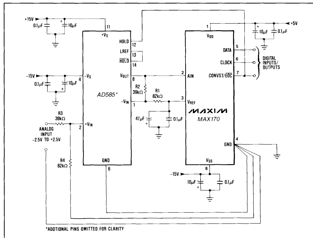
Figure 13. MAX170-AD585 Sample-and-Hold Interface
