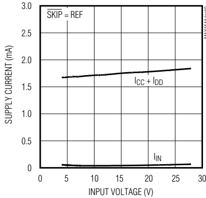
NO-LOAD SUPPLY CURRENT vs. INPUT VOLTAGE (PULSE SKIPPING)
