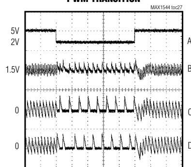
DUAL-PHASE SKIP TO DUAL-PHASE PWM TRANSITION
