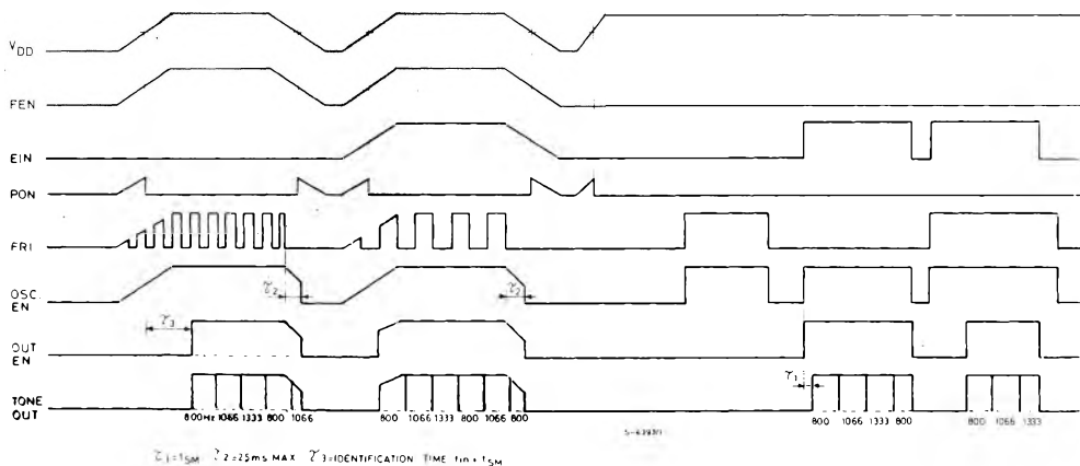
Fig. 3 - Timing diagram
