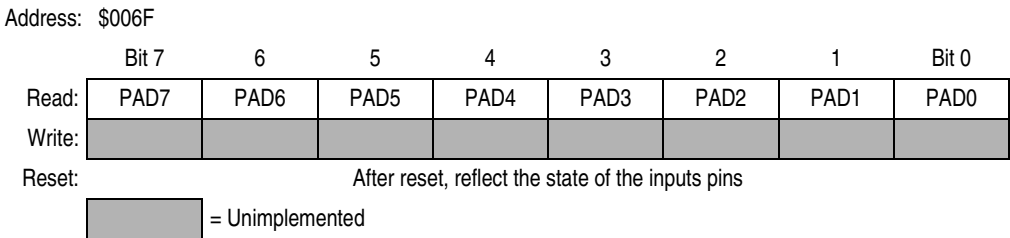
Figure 17-10. Port AD Data Input Register (PORTAD)
