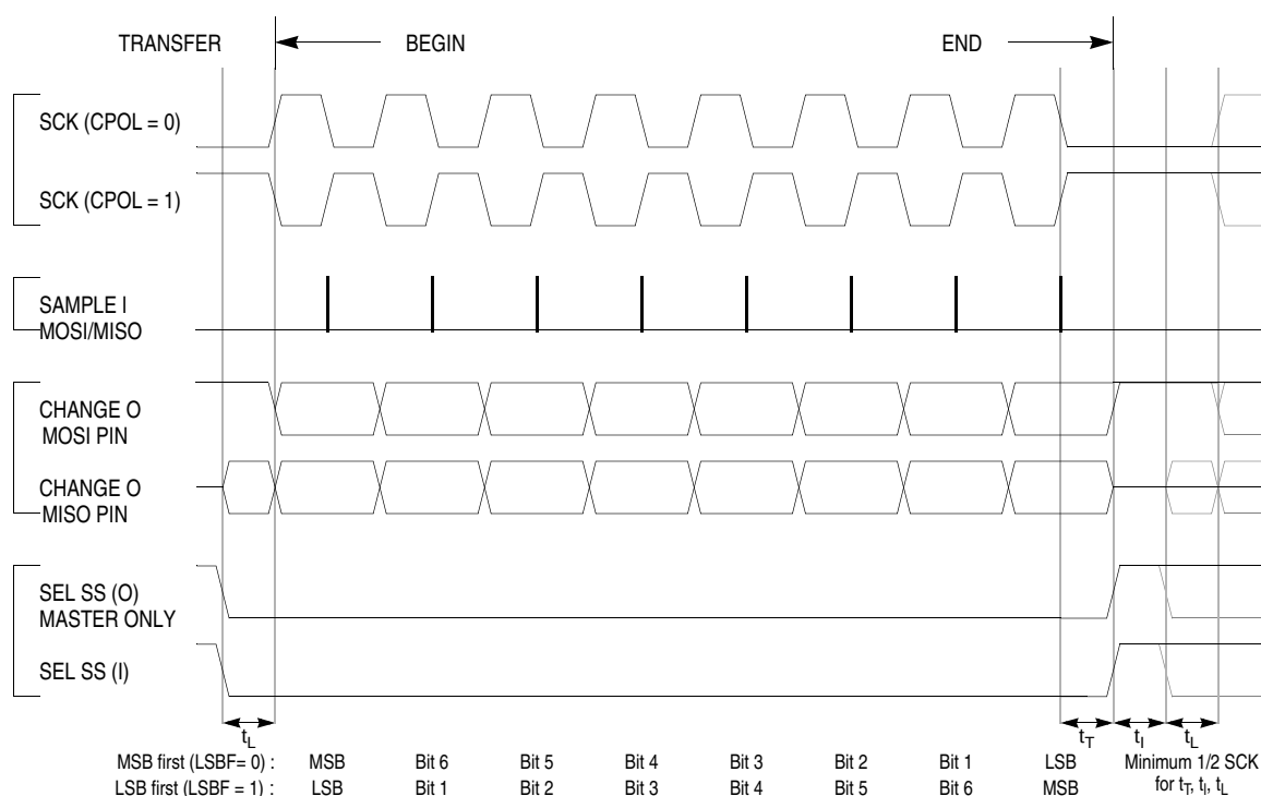
Figure 14-13. SPI Clock Format 1 (CPHA = 1)
