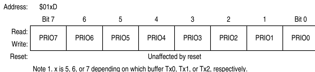
Figure 16-15. Transmit Buffer Priority Register (TBPR)
