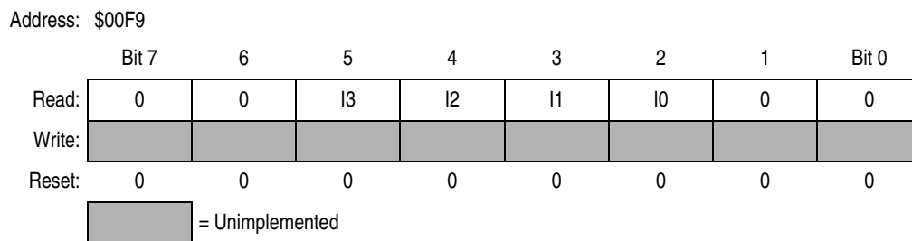
Figure 15-15. BDLC State Vector Register (BSVR)
