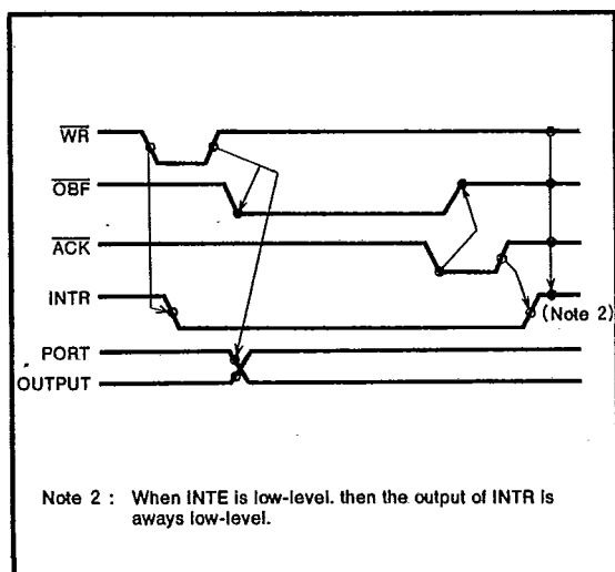
Fig. 6 Timing diagram
