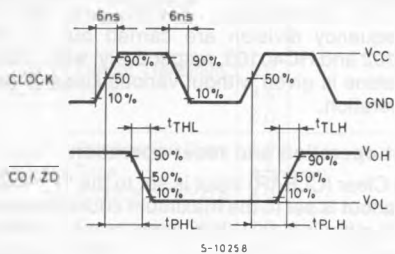
WAVEFORM 1
