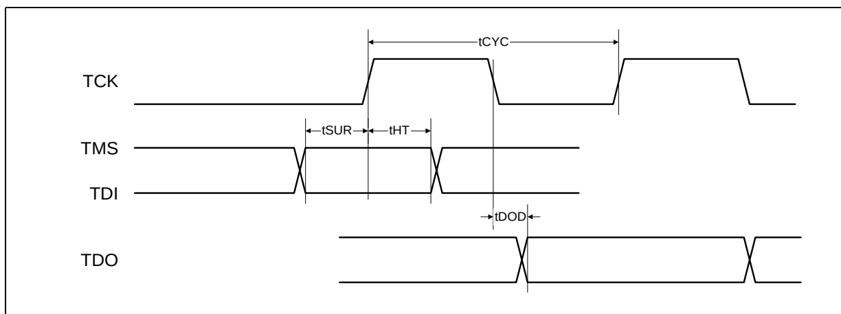
Figure 20. JTAG Timing
