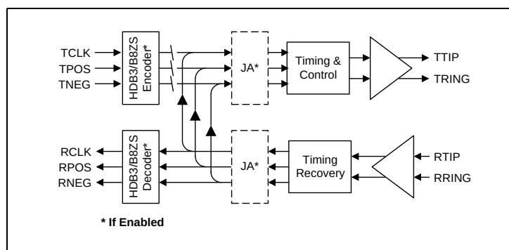
Figure 11. Remote Loopback
