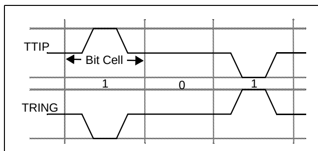
Figure 6. 50% AMI Encoding
