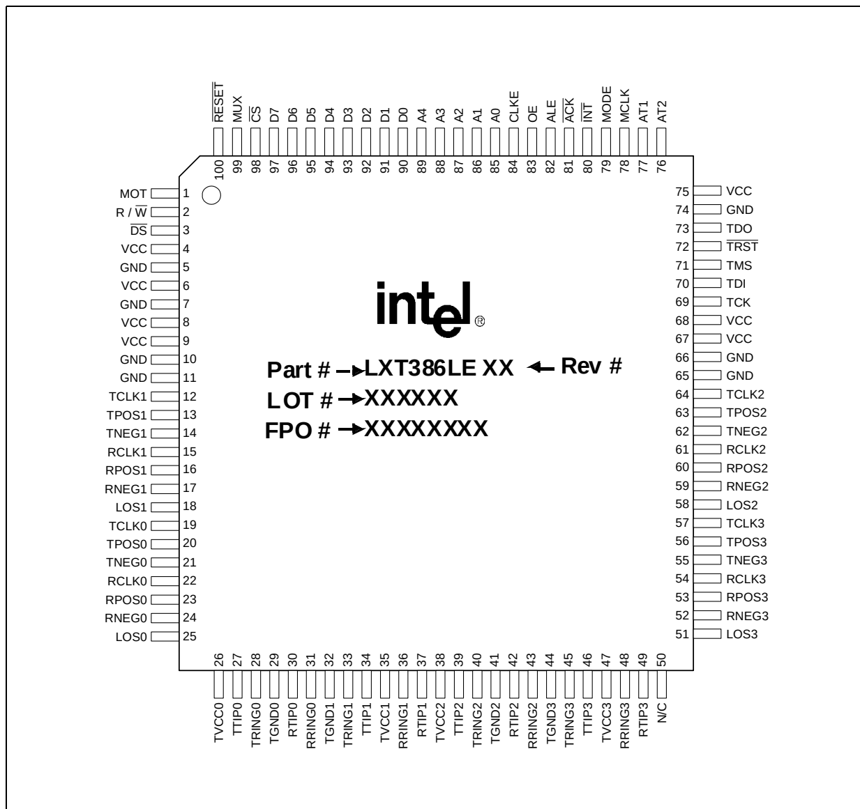
Figure 3. LXT386 Low-Profile Quad Flat Package (LQFP) 100 Pin Assignments and Package Markings
