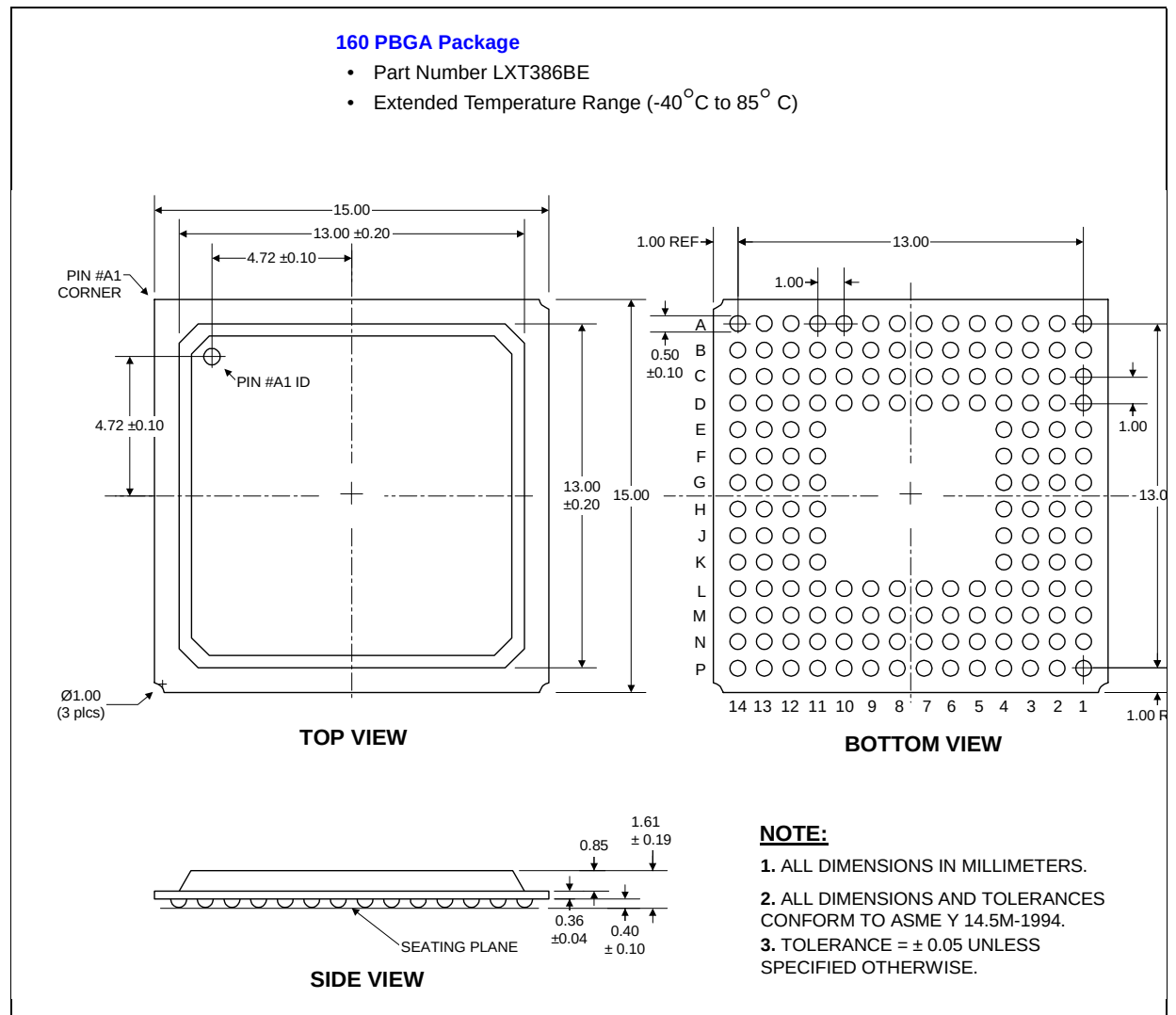
Figure 36. 60 Plastic Ball Grid Array (PBGA) Package Dimensions
