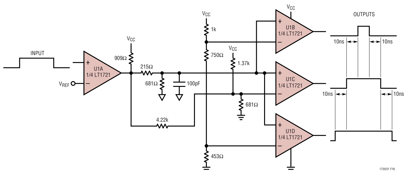
Figure 16. 10ns Triple Overlap Generator
