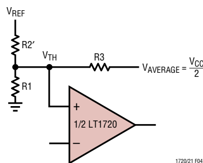
Figure 4. Model for Additional Hysteresis Calculations
