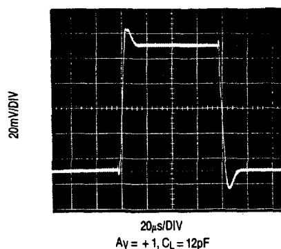
Small Signal Transient Response V_S = \pm 15\text{V}
