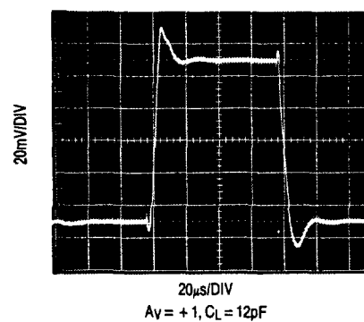
Small Signal Transient Response V_S = \pm 2.5\text{V}
