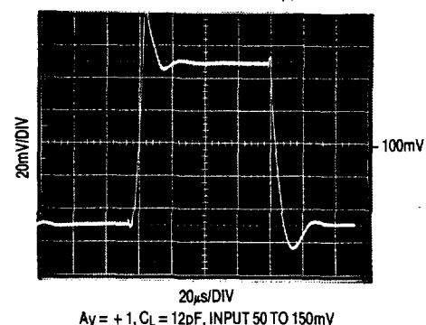
Small Signal Transient Response V_S = 5\text{V}, 0\text{V}
