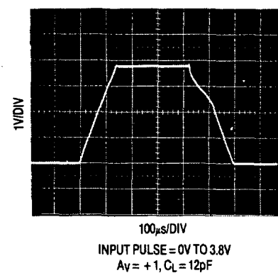
Large Signal Transient Response V_S = 5\text{V}, 0\text{V}
