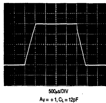
Large Signal Transient Response V_S = \pm 15\text{V}
