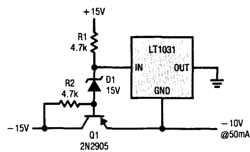
Negative Series Reference
