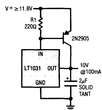
Boosted Output Current With No Current Limit
