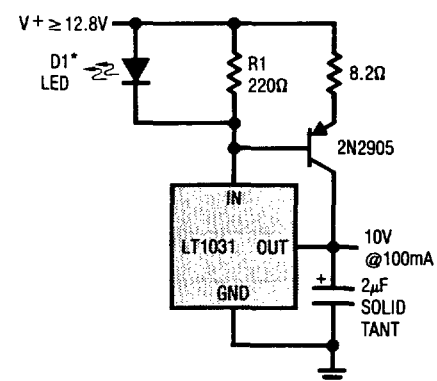
Boosted Output Current With Current Limit
