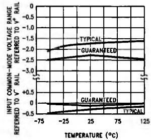
Common-Mode Voltage Range vs Temperature
