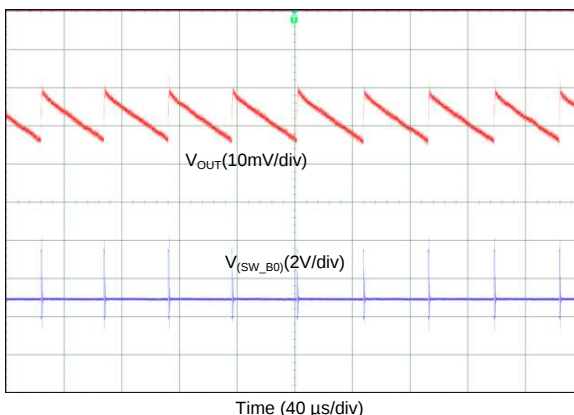
Figure 78. Output Voltage Ripple, PFM Mode (3-Phase Output)
