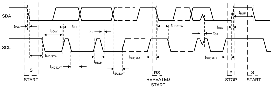
Figure 24. I²C-Compatible Timing
