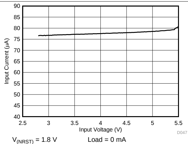
Figure 4. PFM Mode Current Consumption vs Input Voltage (4-Phase Output)
