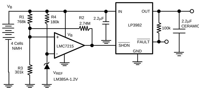
Figure 22. Minimum Battery Detector that Disconnects the Load Via the \overline{\text{SHDN}} Pin of the LP3982
