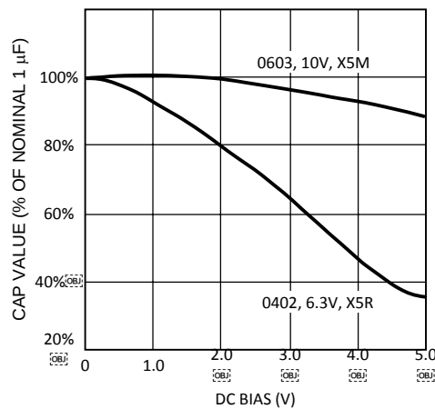
Figure 10. Graph Showing a Typical Variation in Capacitance vs. DC Bias
