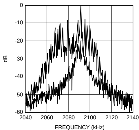
Figure 6. Switching Energy RBW = 300 Hz
