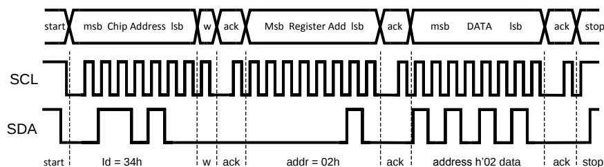
Figure 7. Write cycle
