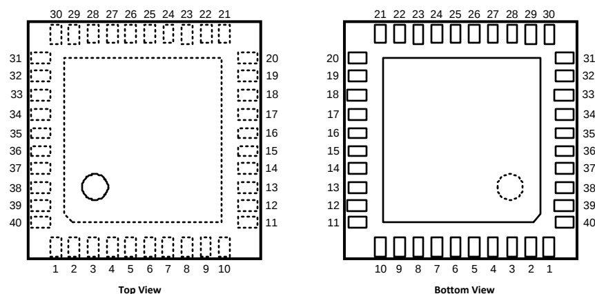
Figure 1. 40-Pin Leadless Leadframe Package
