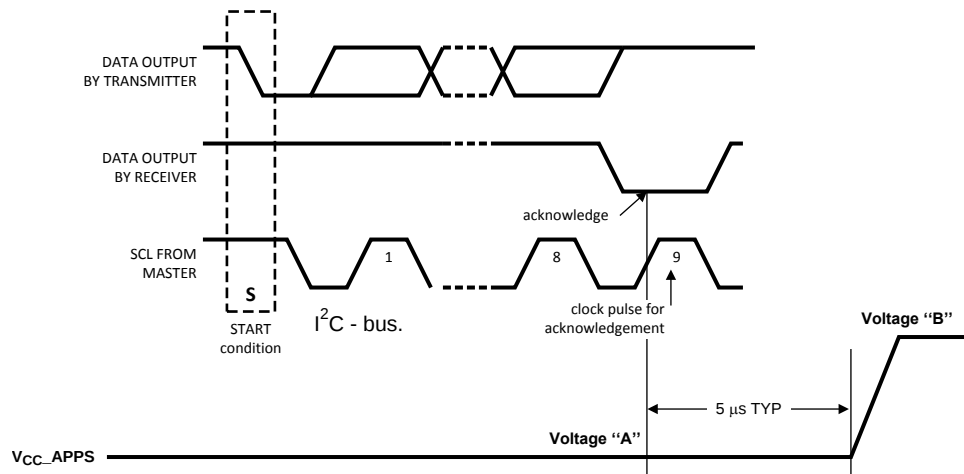
Figure 9. I 2 C DVM Timing for V CC_APPS (Buck1)
