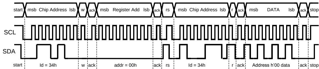
Figure 8. Read Cycle
