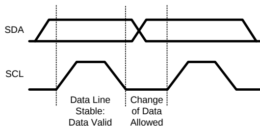
Figure 26. Bit Transfer
