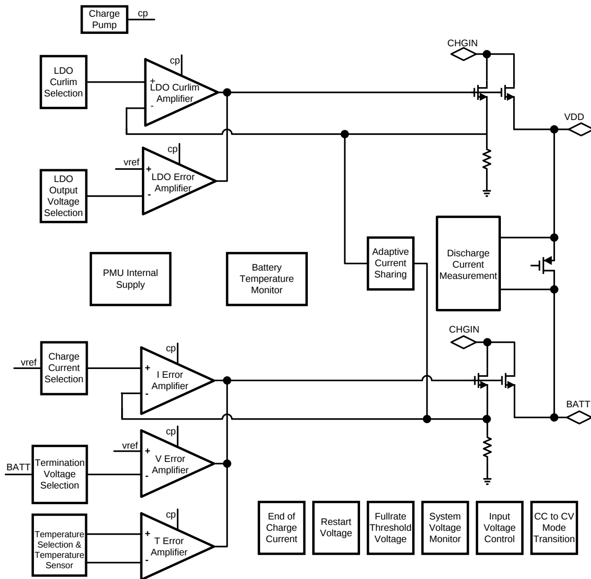
Figure 9. Charger Block Diagram
