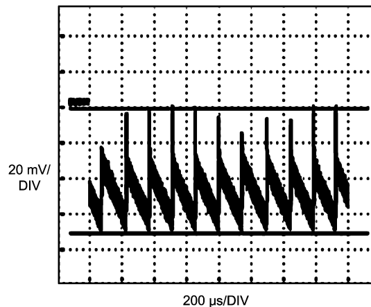
Figure 15. Typical Ripple in ECO Mode
