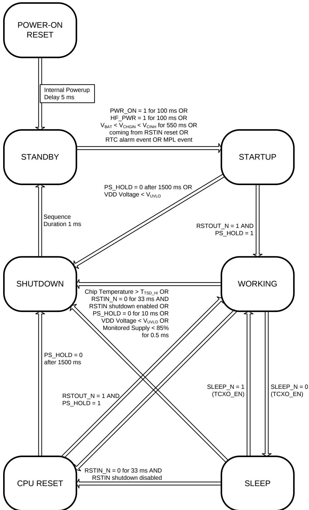
Figure 2. Device Operating Modes
