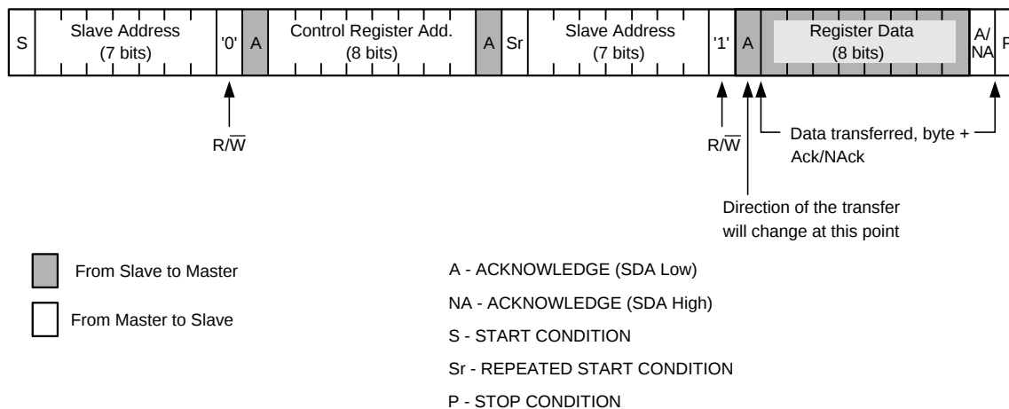
Figure 30. Register Read Format
