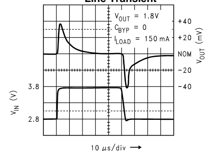
Line Transient
