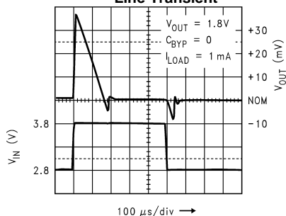
Line Transient
