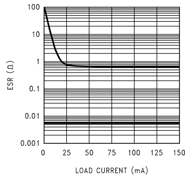
Figure 4. LP2985LV 4.7µF Stable ESR Range
