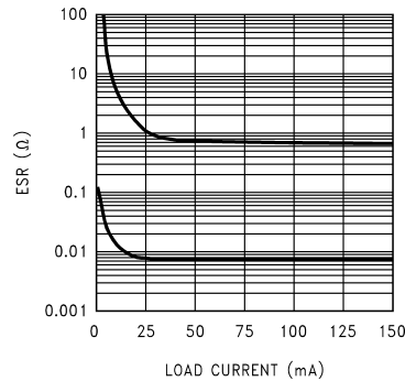
Figure 3. LP2985LV 2.2µF Stable ESR Range
