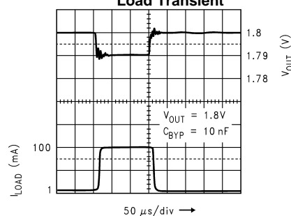
Load Transient
