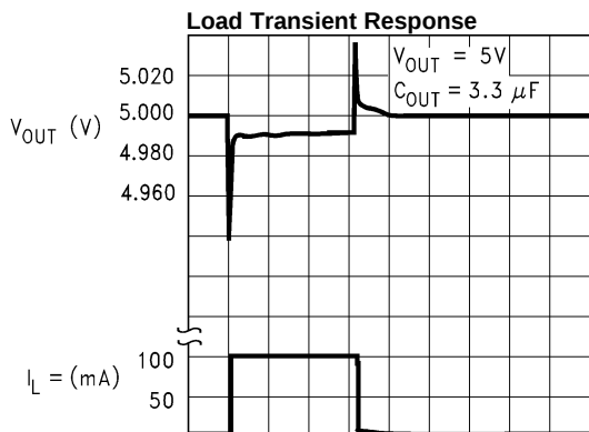
10 \mu\text{s}/\text{div} → Figure 18.
