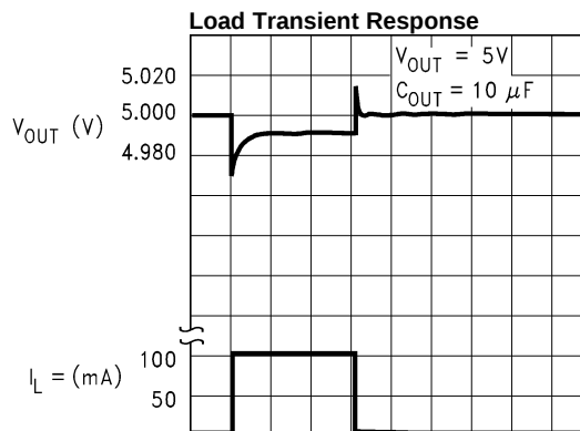
10 \mu\text{s}/\text{div} → Figure 19.
