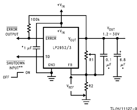
FIGURE 4. Adjustable Regulator
