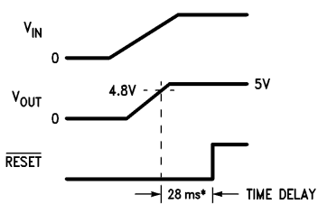
Timing Diagram for Timed Power-On Reset
