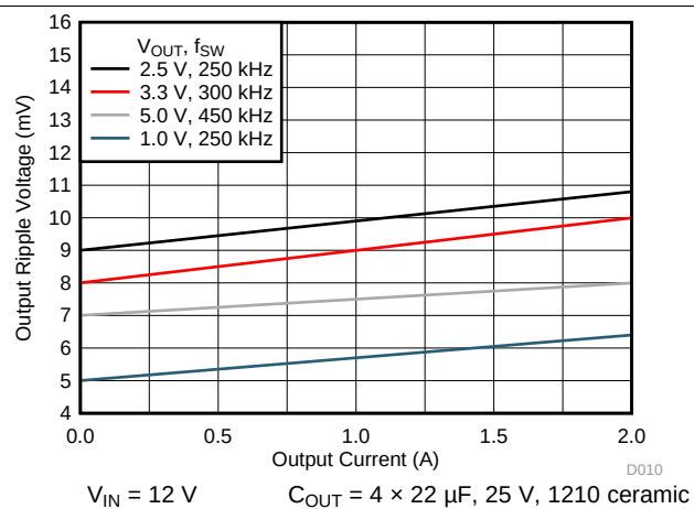
Figure 7. Voltage Ripple vs Output Current
