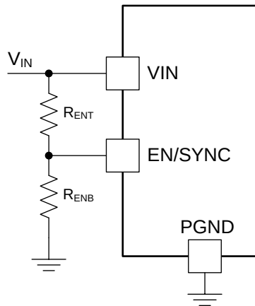
Figure 26. Adjustable UVLO
