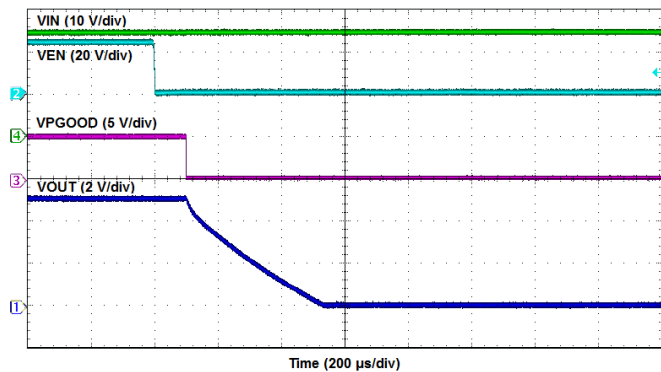
Figure 25. Enable Turn-OFF
