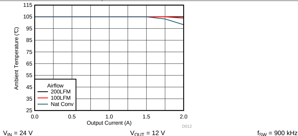
Figure 13. Safe Operating Area
