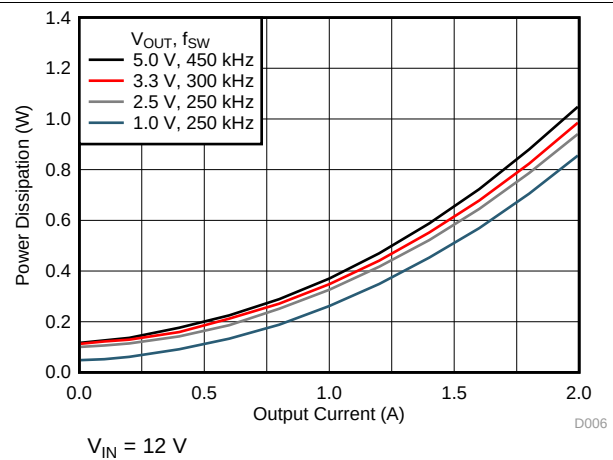
Figure 6. Power Dissipation vs Output Current
