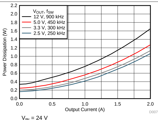
Figure 10. Power Dissipation vs Output Current
