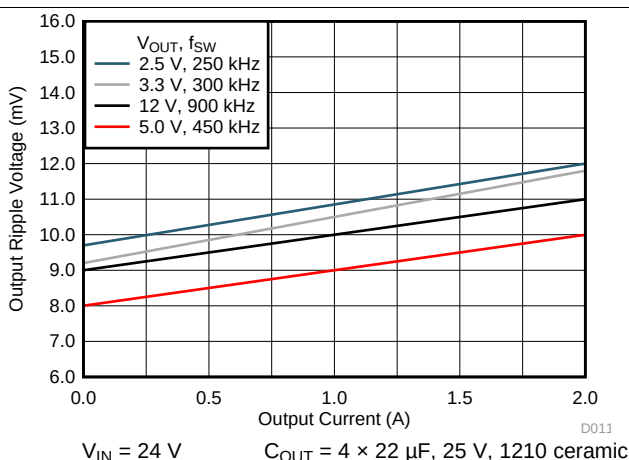
Figure 11. Voltage Ripple vs Output Current
