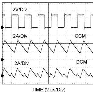
Figure 9. CCM and DCM Operating Modes V_{IN} = 12\text{V} , V_O = 3.3\text{V} , I_O = 3\text{A}/0.3\text{A}
