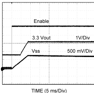
Figure 8. Pre-Biased Startup
