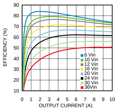
Efficiency 1.0V output @ 85°C
