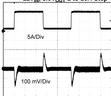
TIME (500 μs/Div) Figure 44.
