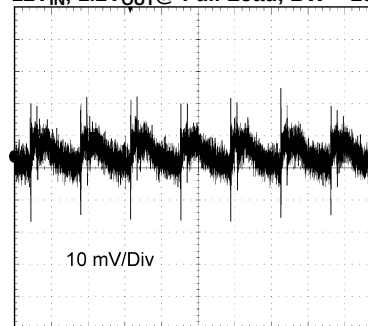
TIME (2 μs/Div) Figure 43.
