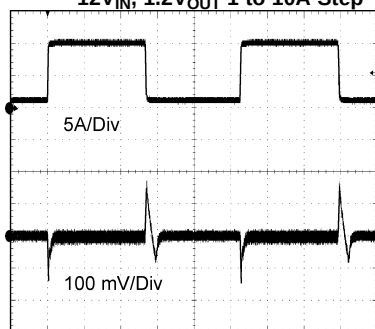
TIME (500 μs/Div) Figure 46.
