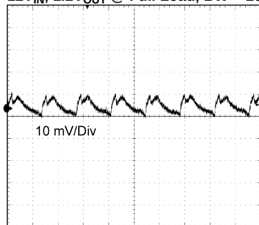
TIME (2 μs/Div) Figure 42.
