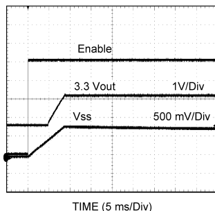
Figure 53. Pre-Biased Startup
