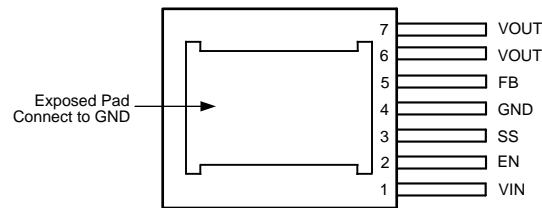
Figure 2. Top View 7-Lead PFM Package Number NDW0007A
