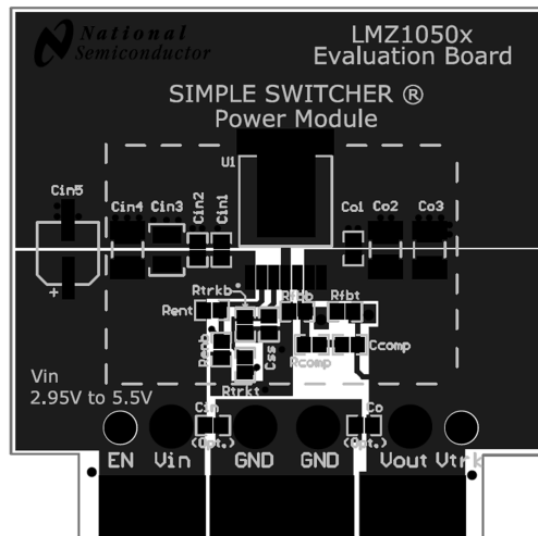
Figure 20. Top Copper
