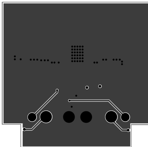
Figure 22. Internal Layer 2 (Ground and Signal Traces)
