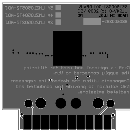
Figure 23. Bottom Copper
