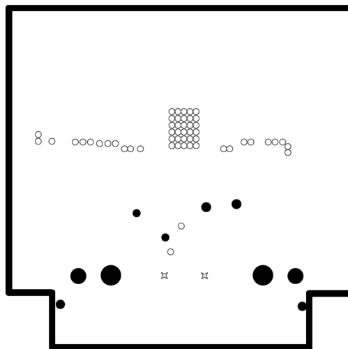
Figure 21. Internal Layer 1 (Ground)
