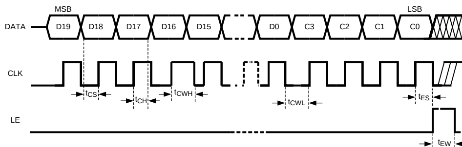
Figure 2. MICROWIRE Input Timing Diagram
