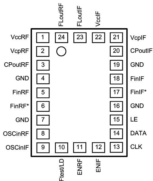
Ultra Thin 24-Pin CSP (SLE) Package
