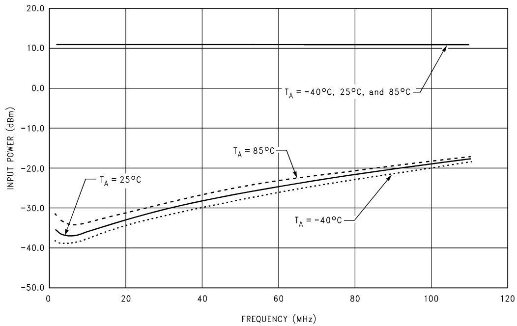
OSCinRF Counter Sensitivity V_{CC} = 3.0\text{V}
