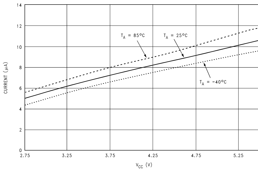
Powerdown Current V_{ENRF} = V_{ENIF} = 0\text{V}
