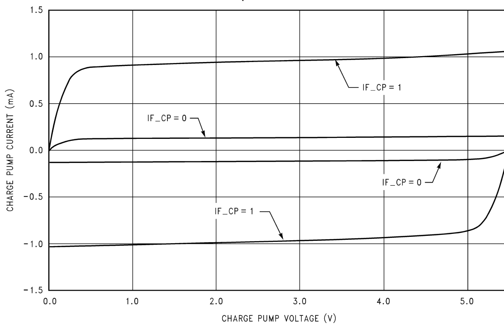
IF Charge Pump Current V_{VCP\text{IF}} = 5.0\text{V}
