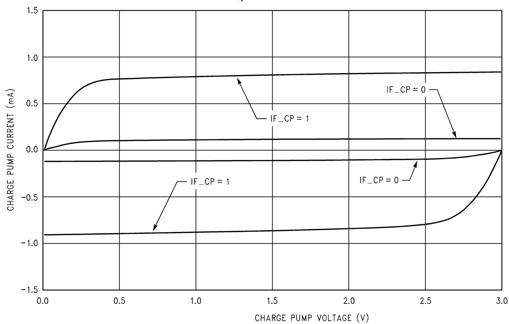
IF Charge Pump Current V_{VCP\text{IF}} = 3.0\text{V}
