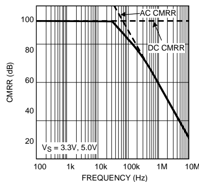
Figure 6. CMRR Curve
