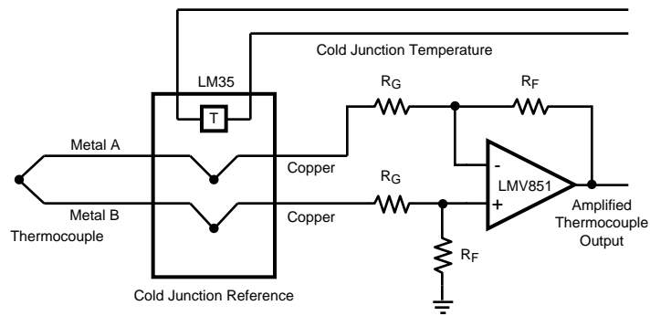
Figure 13. Thermocouple Read Out Circuit
