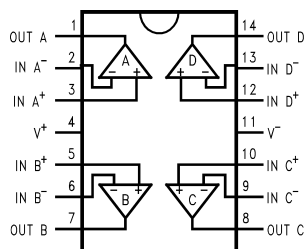
Figure 4. 14-Pin TSSOP (Top View)
