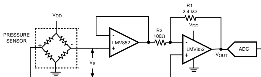
Figure 11. Pressure Sensor Application
