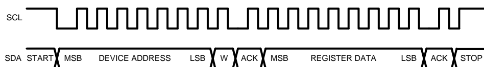
Figure 11. Start and Stop Diagram
