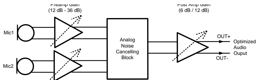
Figure 7. Simplified Block Diagram of the LMV1099 Uplink path
