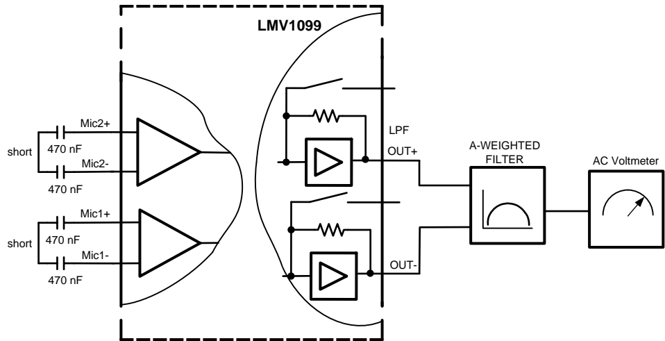
Figure 16. Noise Measurement Setup
