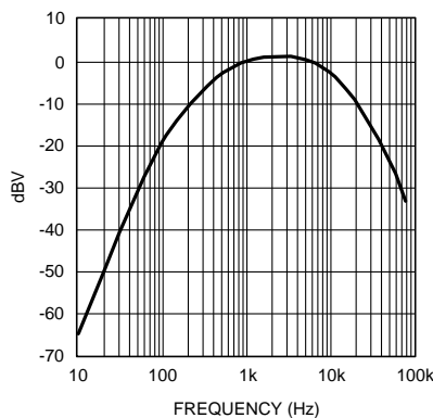
Figure 15. A-Weighted Filter
