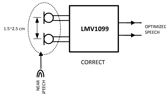
Figure 14. Endfire Array (CORRECT)
