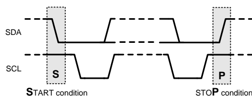
Figure 10. I 2 C Start Stop Conditions
