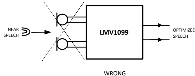
Figure 13. Broadside Array (WRONG)
