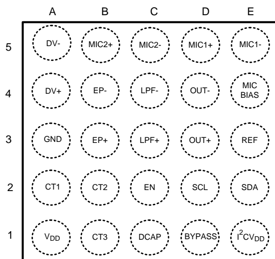
Figure 3. Top View 25 – Bump micro SMD Package
