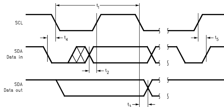
Figure 9. I 2 C Timing Diagram
