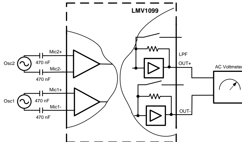
Figure 6. FFNS E , NFSL E , SNRI E Test Circuit
