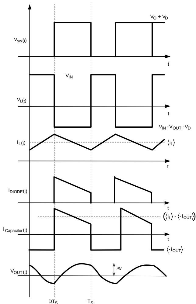
Figure 14. Typical Waveforms
