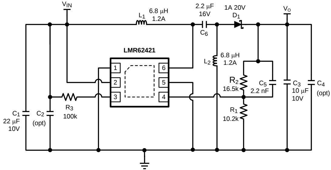
Figure 28. V_{in} = 2.7\text{V} - 5\text{V} , V_{out} = 3.3\text{V} @ 500mA
