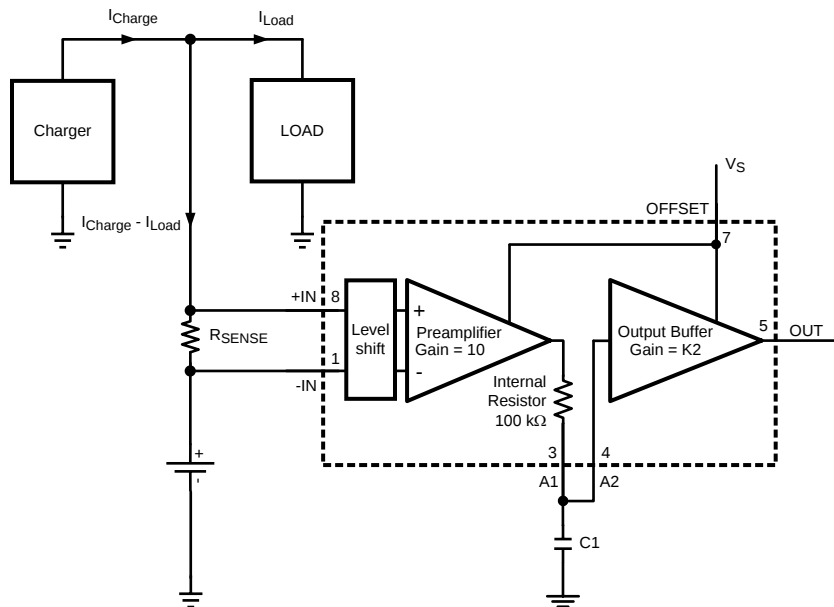
Figure 14. Battery Current Monitor Application
