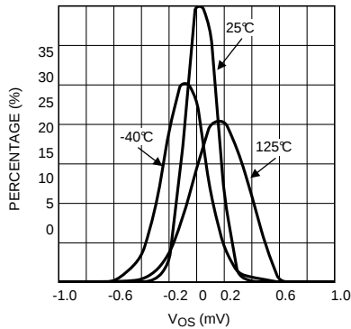
V_{\text{OS}} Distribution at V_S = 3.3\text{V} 5000 parts
