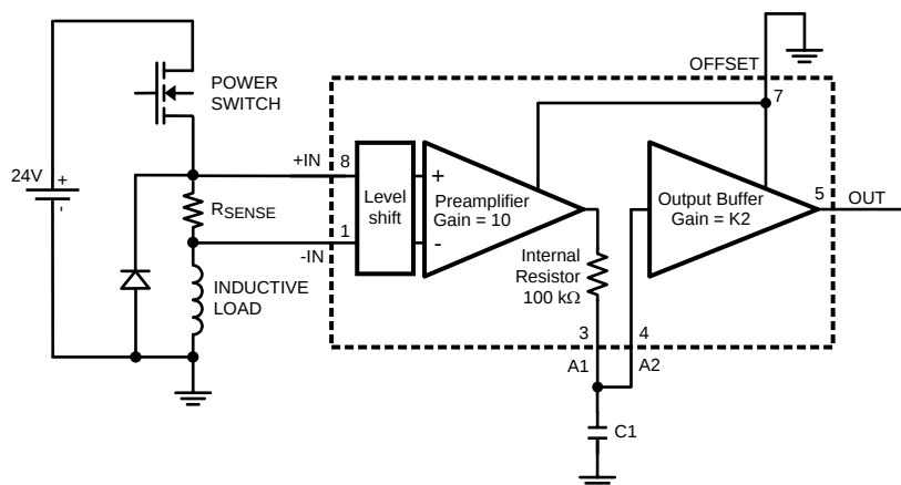
Figure 13. High Side Current Sensing Application with Negative Common Mode Transients
