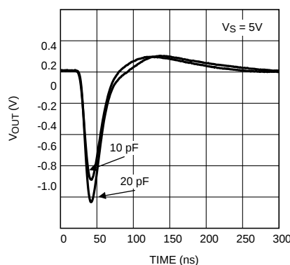
Figure 10. Capacitive Load Response at 5.0V
