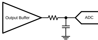
Figure 11. Reduce Error When Driving ADCs
