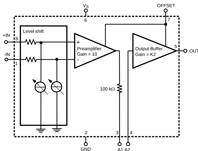
Figure 3. Theory of Operation
