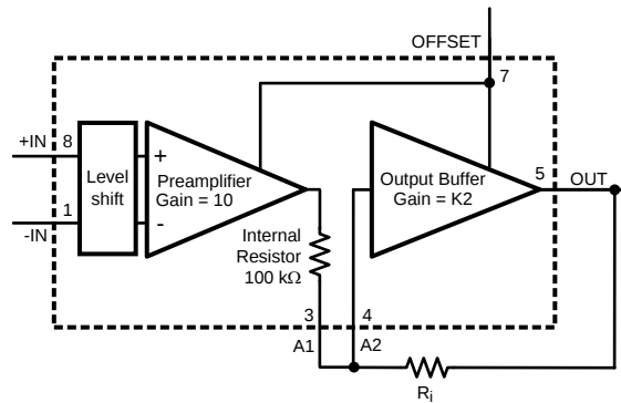
Figure 7. Increase Gain
