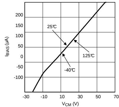
Input Bias Current Over Temperature (A2 pin) at V_S = 5\text{V}
