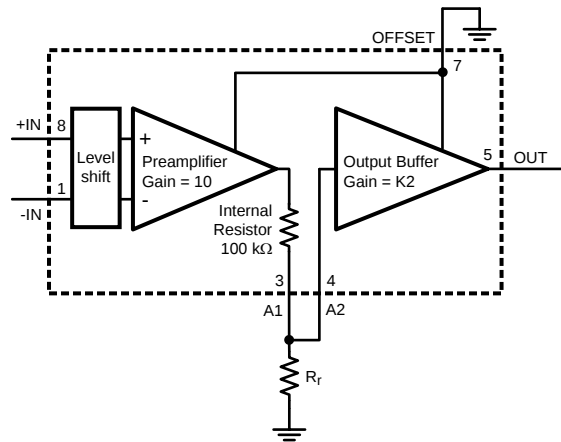
Figure 5. Reduce Gain for Unidirectional Application
