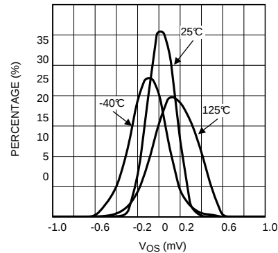
V_{\text{OS}} Distribution at V_S = 5\text{V} 5000 parts
