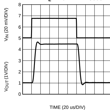
Settling Time (Falling Edge) at V_S = 5\text{V} LMP8603
