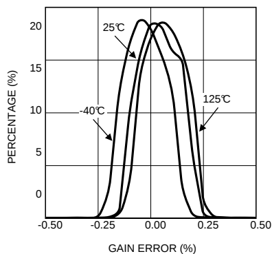
Gain error Distribution at V_S = 5\text{V} LMP8602 5000 parts
