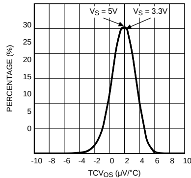
\text{TCV}_{\text{OS}} Distribution 5000 parts
