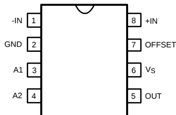
Figure 2. Top View
