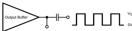
Figure 8. Driving Switched Capacitive Load
