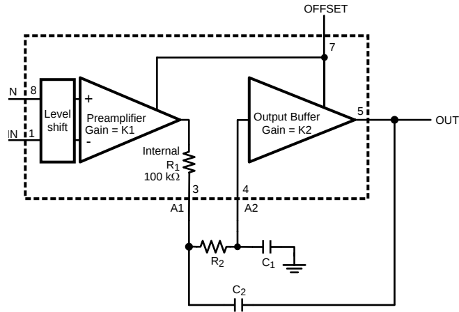
Figure 4. Second Order Low Pass Filter
