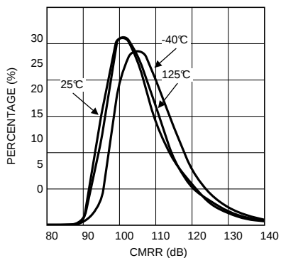
CMRR Distribution at V_S = 3.3\text{V} 5000 parts
