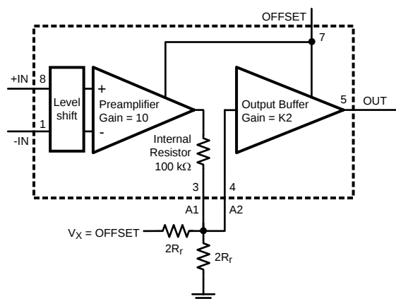
Figure 6. Reduce Gain for Bidirectional Application
