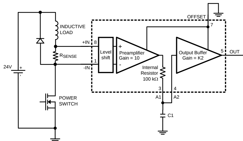
Figure 12. Low Side Current Sensing Application with Large Common Mode Transients
