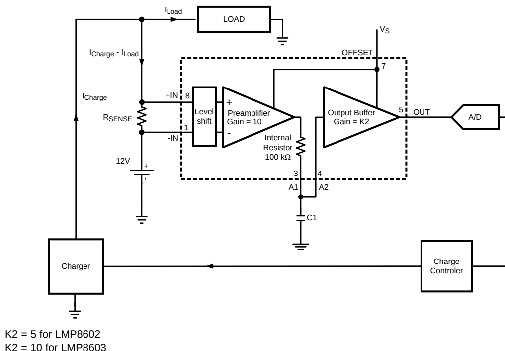
Figure 15. Advanced Battery Charger Application
