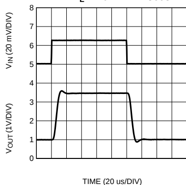
Settling Time (Falling Edge) at V_S = 3.3\text{V} LMP8603
