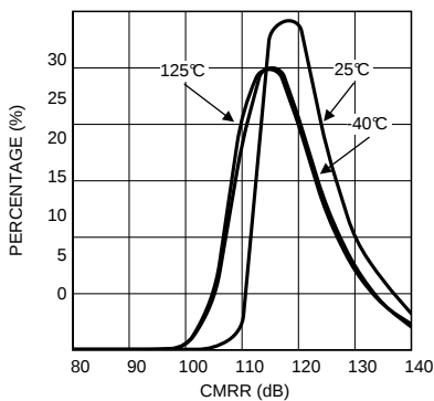
CMRR Distribution at V_S = 5\text{V} 5000 parts
