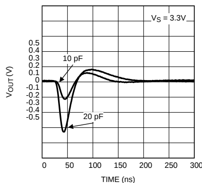
Figure 9. Capacitive Load Response at 3.3V
